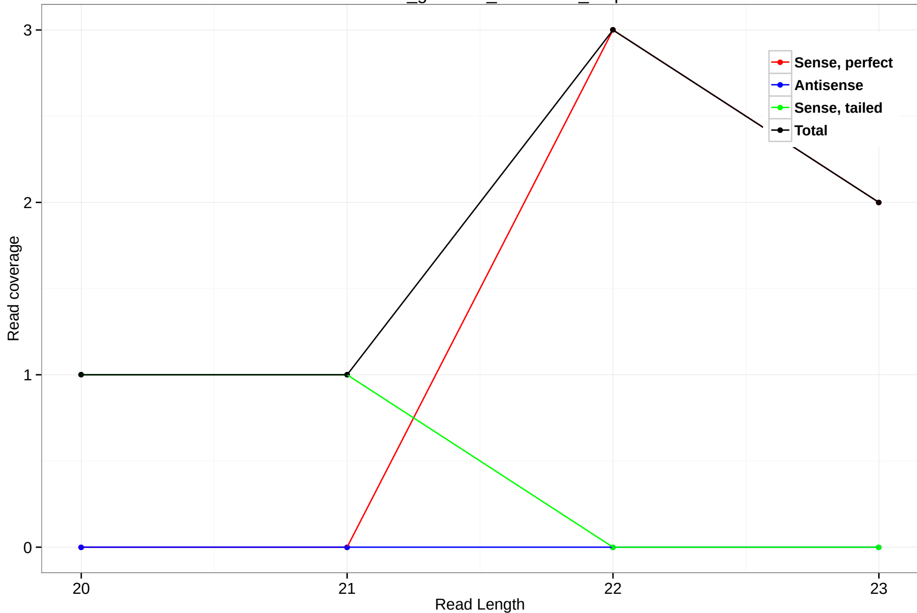
rheMac3_genscan_chr7.3259_2.3p
