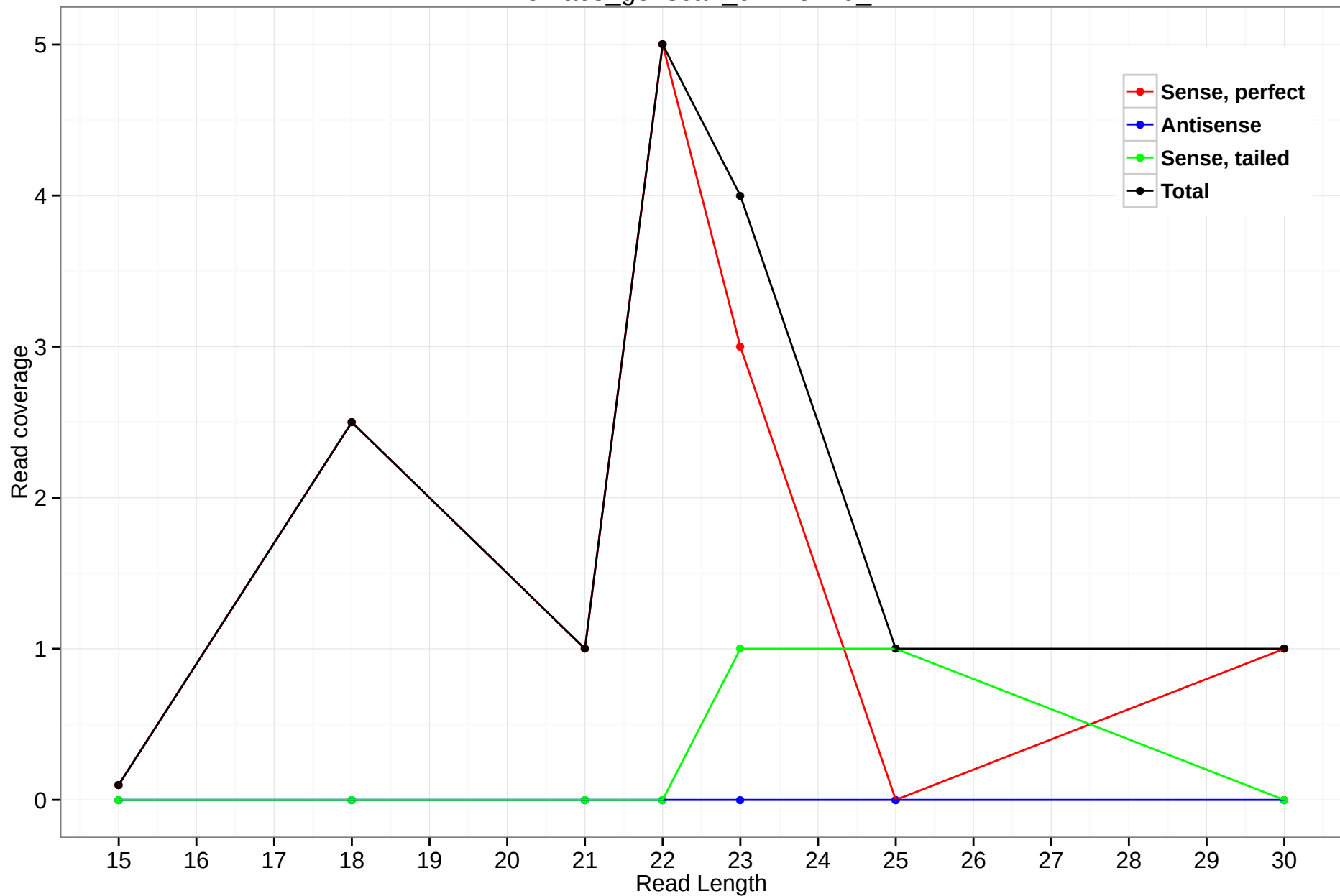
rheMac3_genscan_chr7.3249_11
