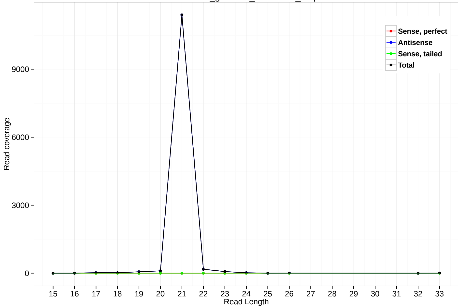
rheMac3_genscan_chr7.3189_9.3p
