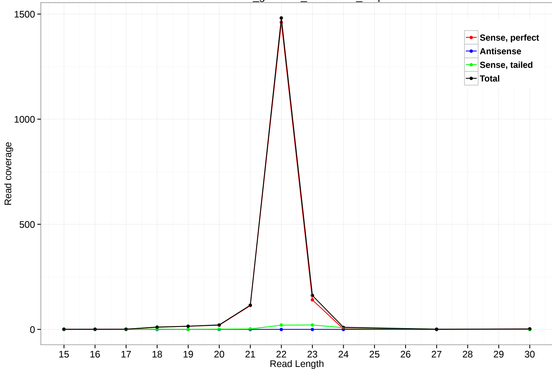
rheMac3_genscan_chr7.3188_4.5p
