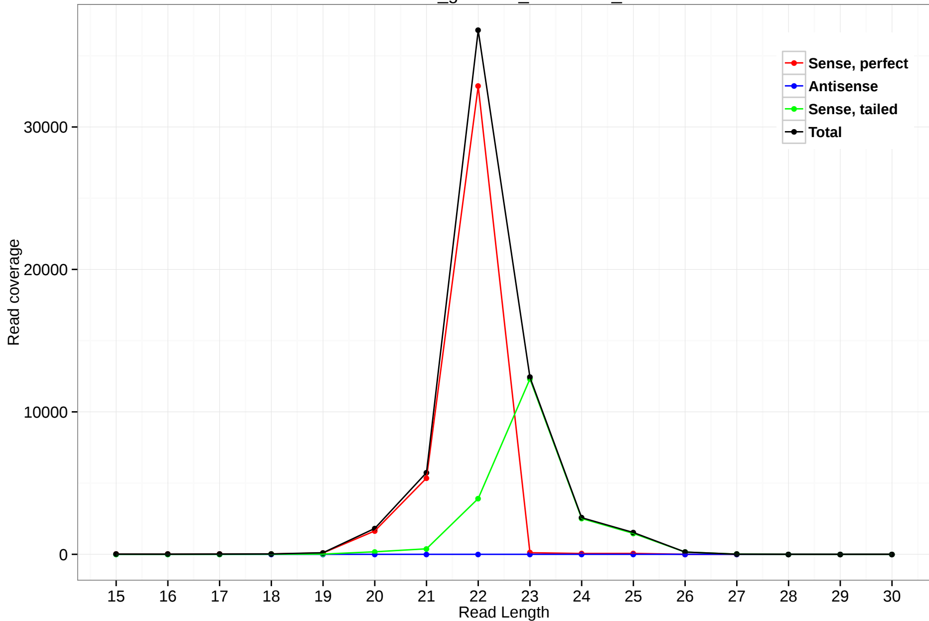
rheMac3_genscan_chr7.3188_11
