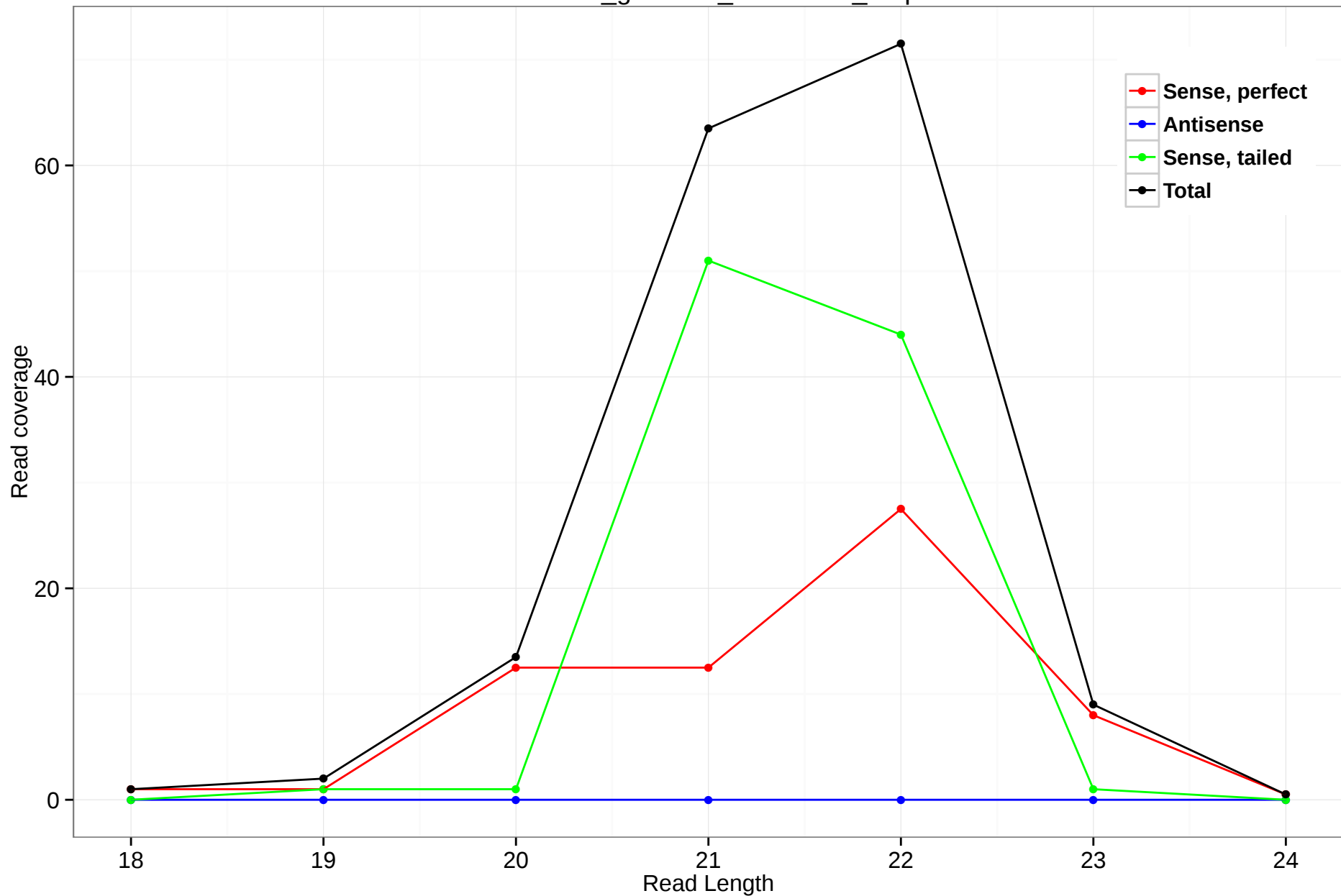
rheMac3_genscan_chr7.3188_0.5p
