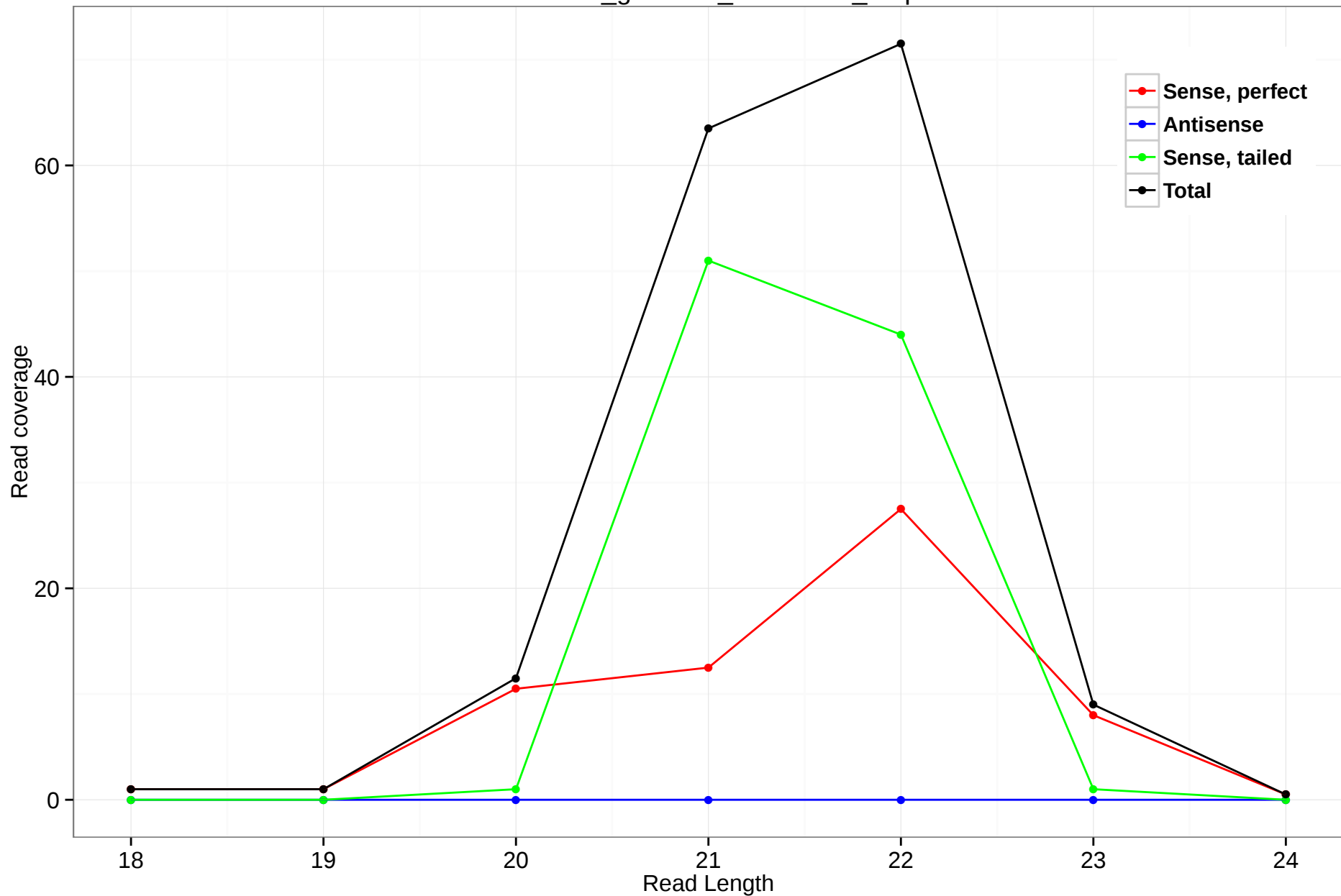
rheMac3_genscan_chr7.3188_0.3p
