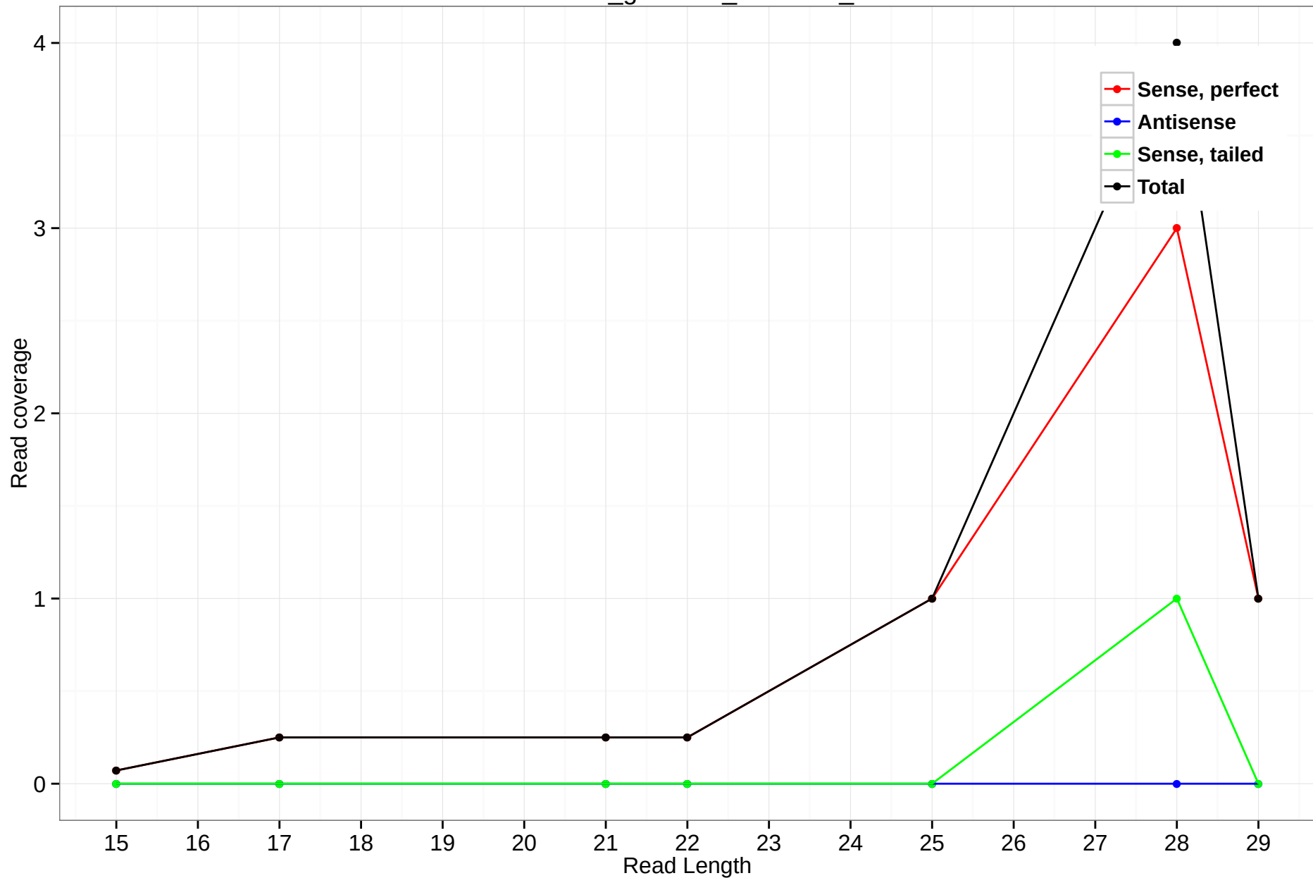
rheMac3_genscan_chr7.314_0
