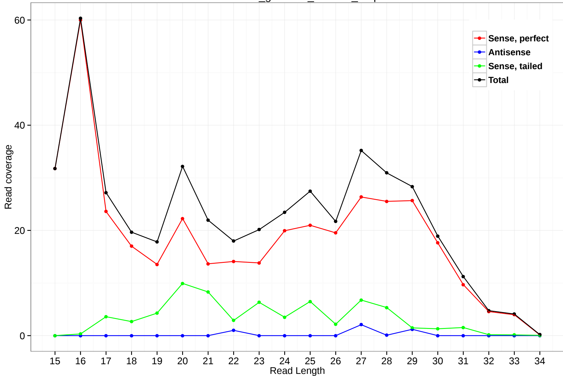
rheMac3_genscan_chr7.30_6.5p
