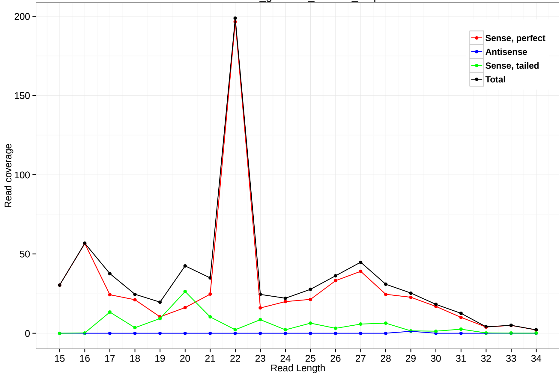
rheMac3_genscan_chr7.30_4.5p
