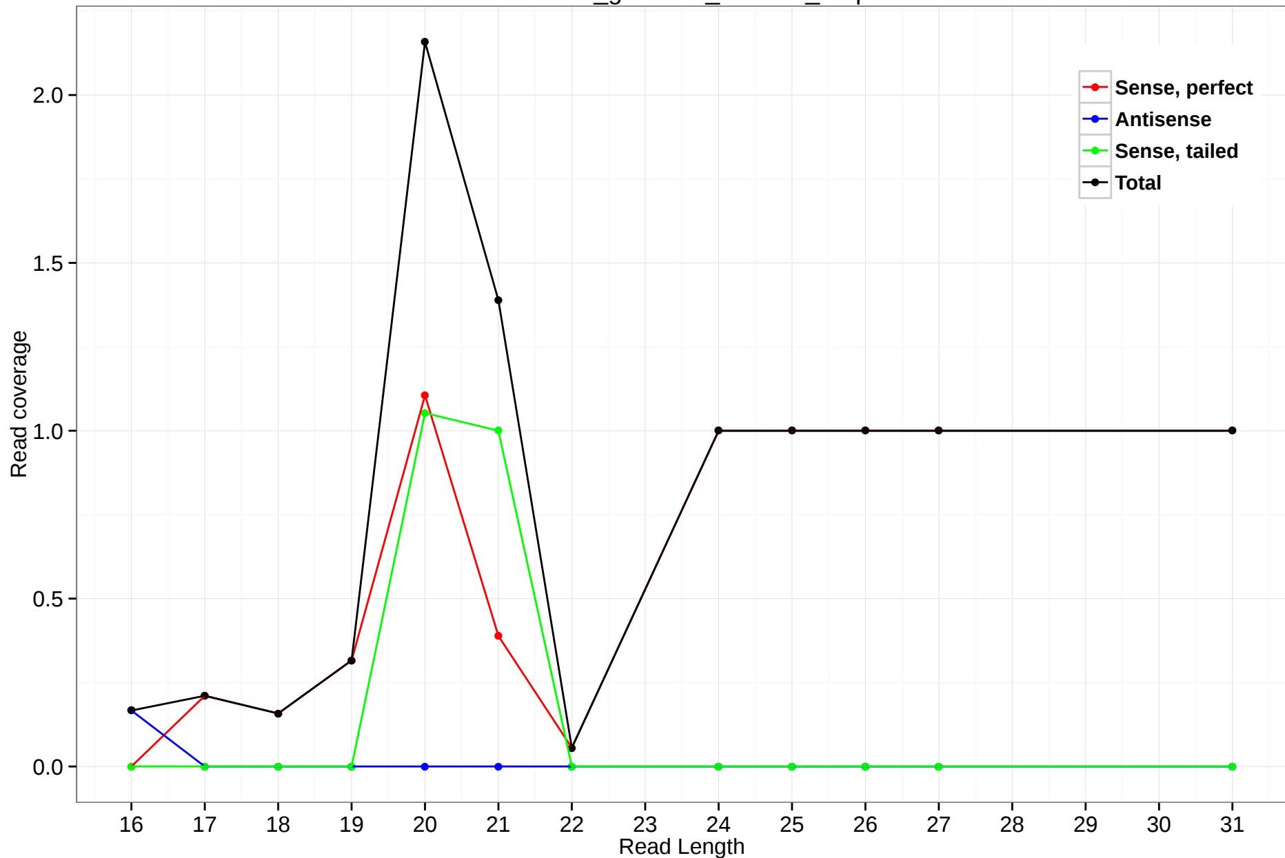
rheMac3_genscan_chr7.30_3.5p
