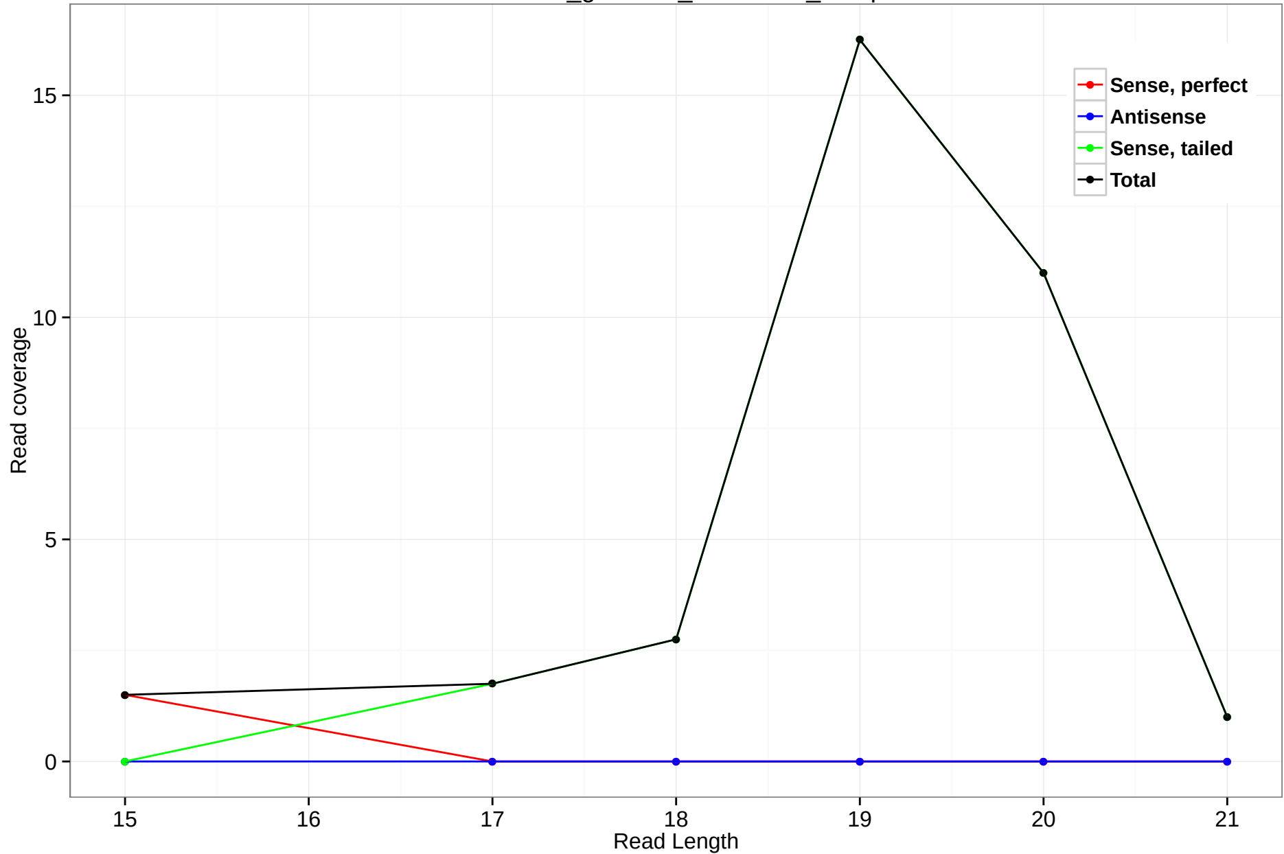
rheMac3_genscan_chr7.2979_28.5p
