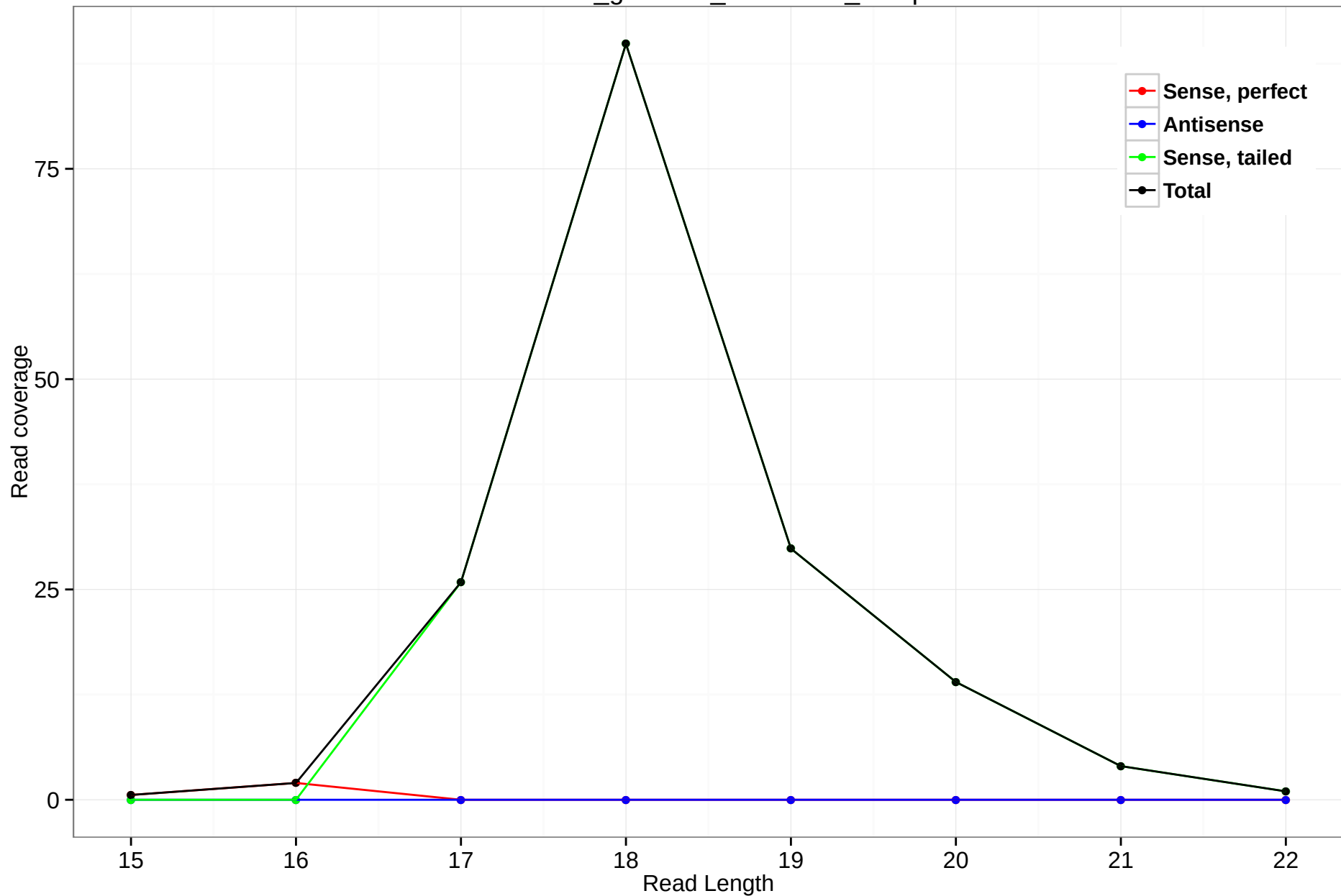
rheMac3_genscan_chr7.2780_16.5p
