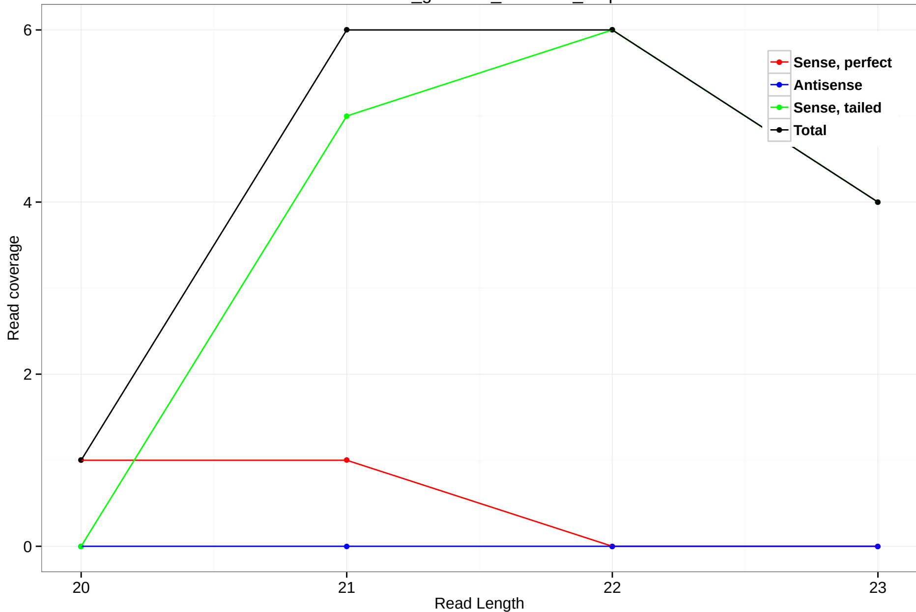
rheMac3_genscan_chr7.277_0.5p
