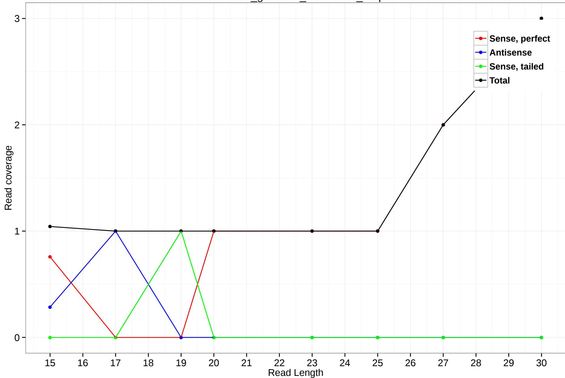
rheMac3_genscan_chr7.2707_6.5p
