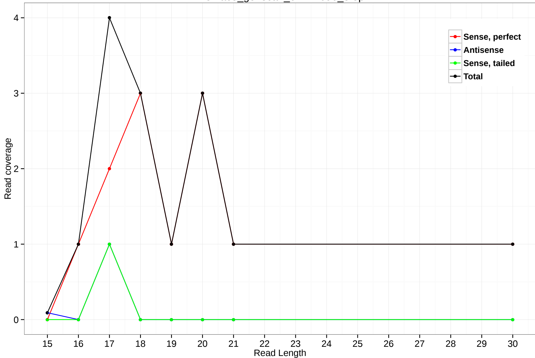
rheMac3_genscan_chr7.2696_3.3p
