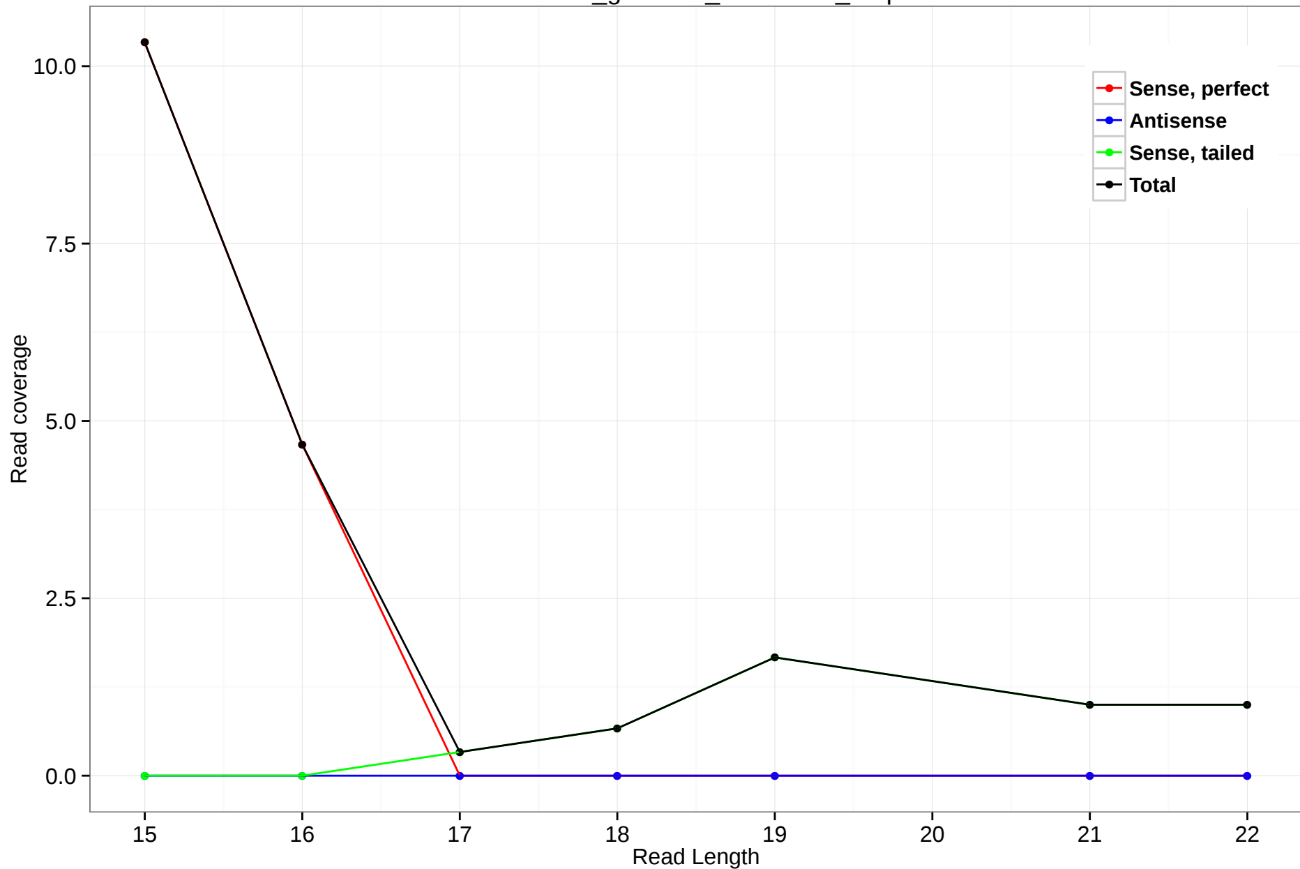
rheMac3_genscan_chr7.2693_2.3p
