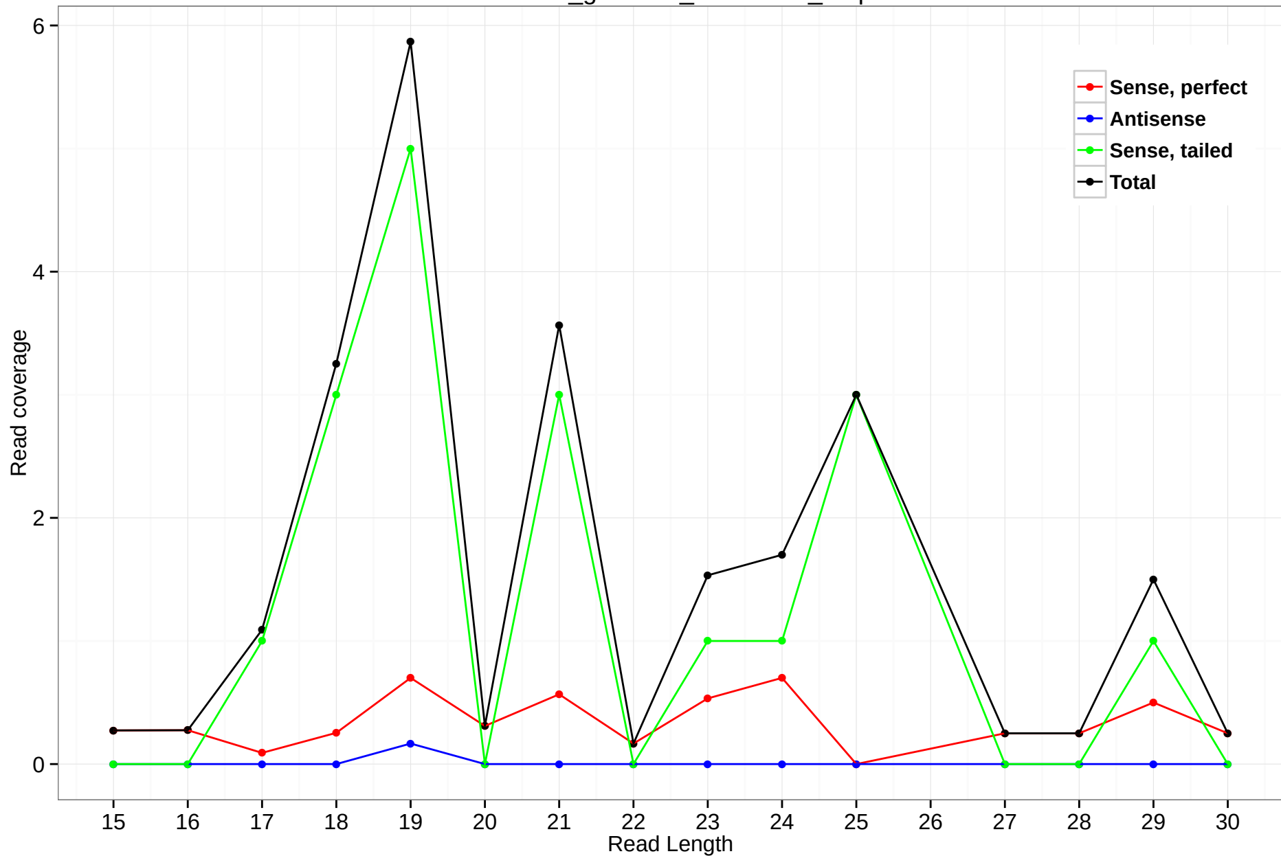
rheMac3_genscan_chr7.2650_1.3p
