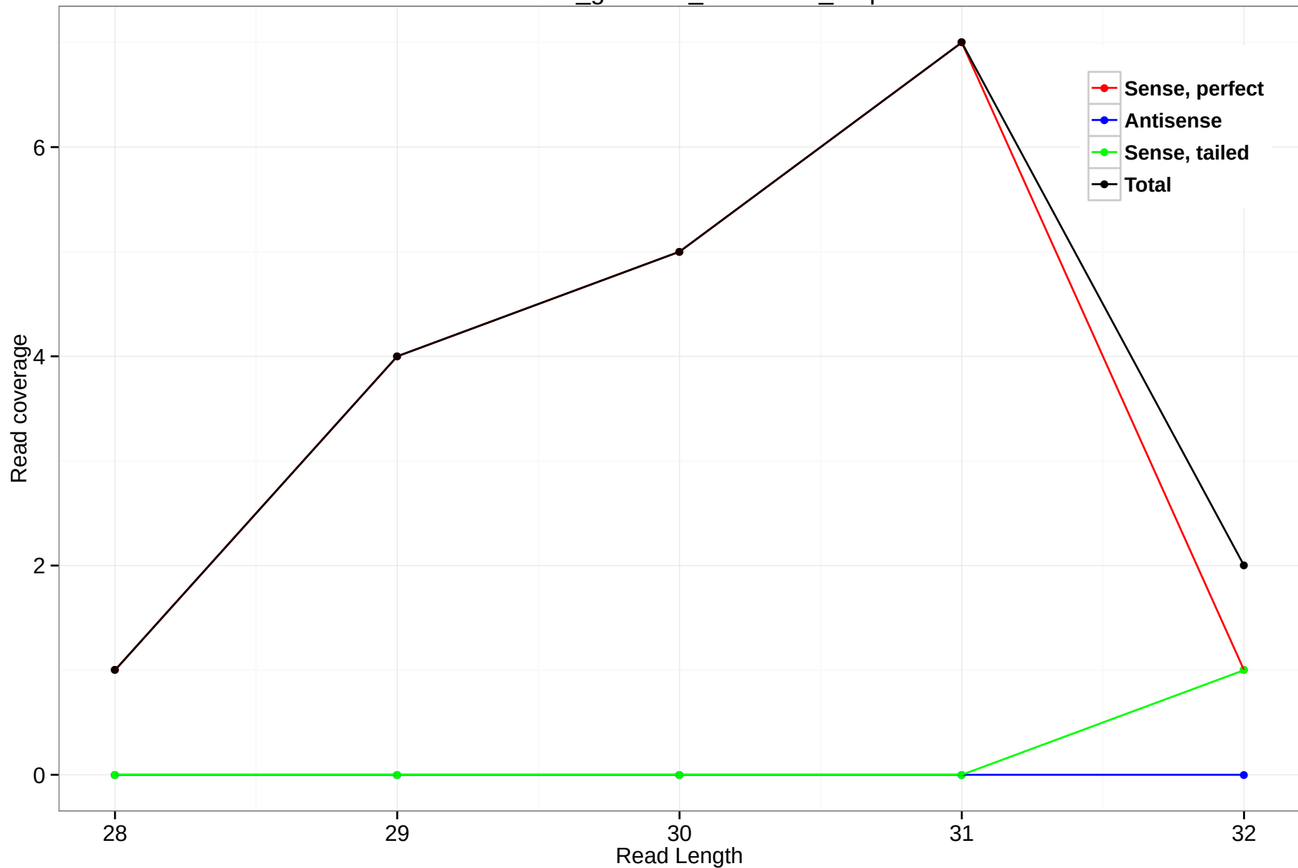
rheMac3_genscan_chr7.2641_1.3p
