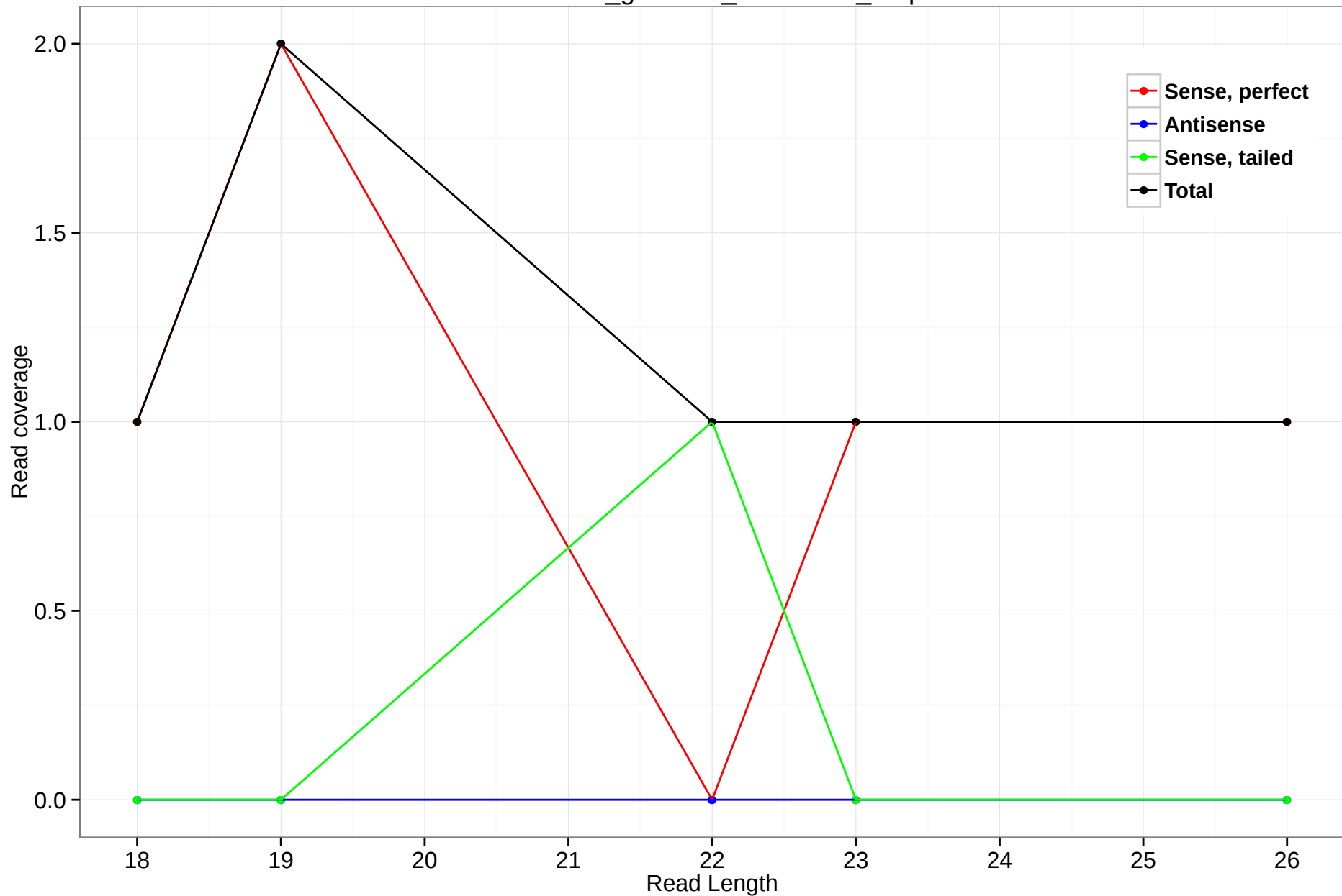
rheMac3_genscan_chr7.2606_9.3p
