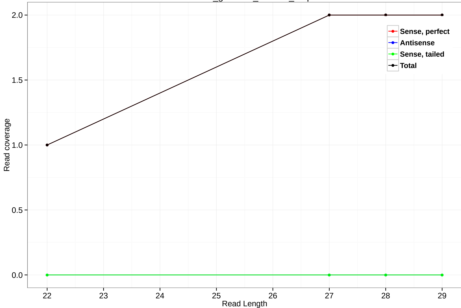
rheMac3_genscan_chr7.25_3.5p
