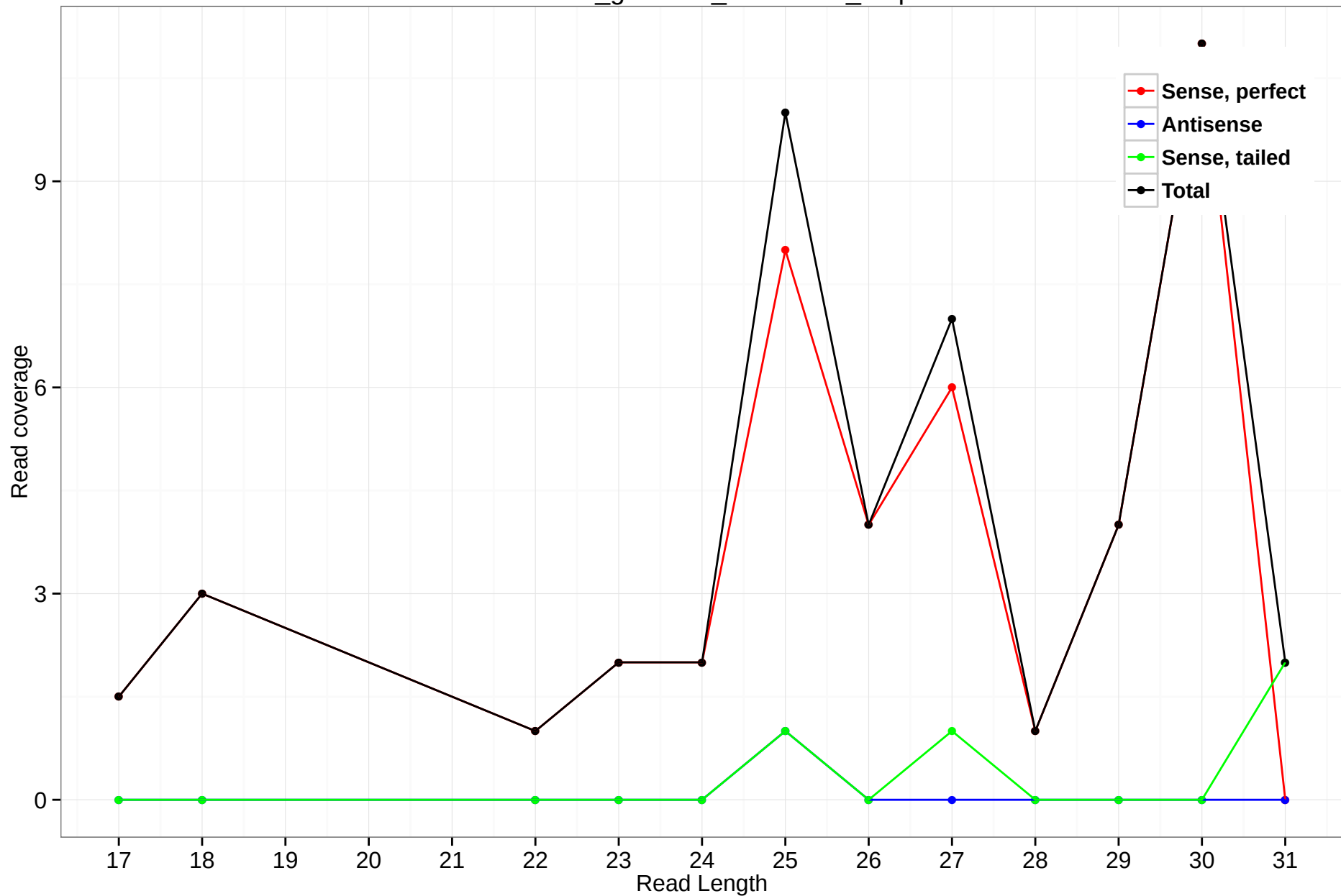
rheMac3_genscan_chr7.2576_4.3p
