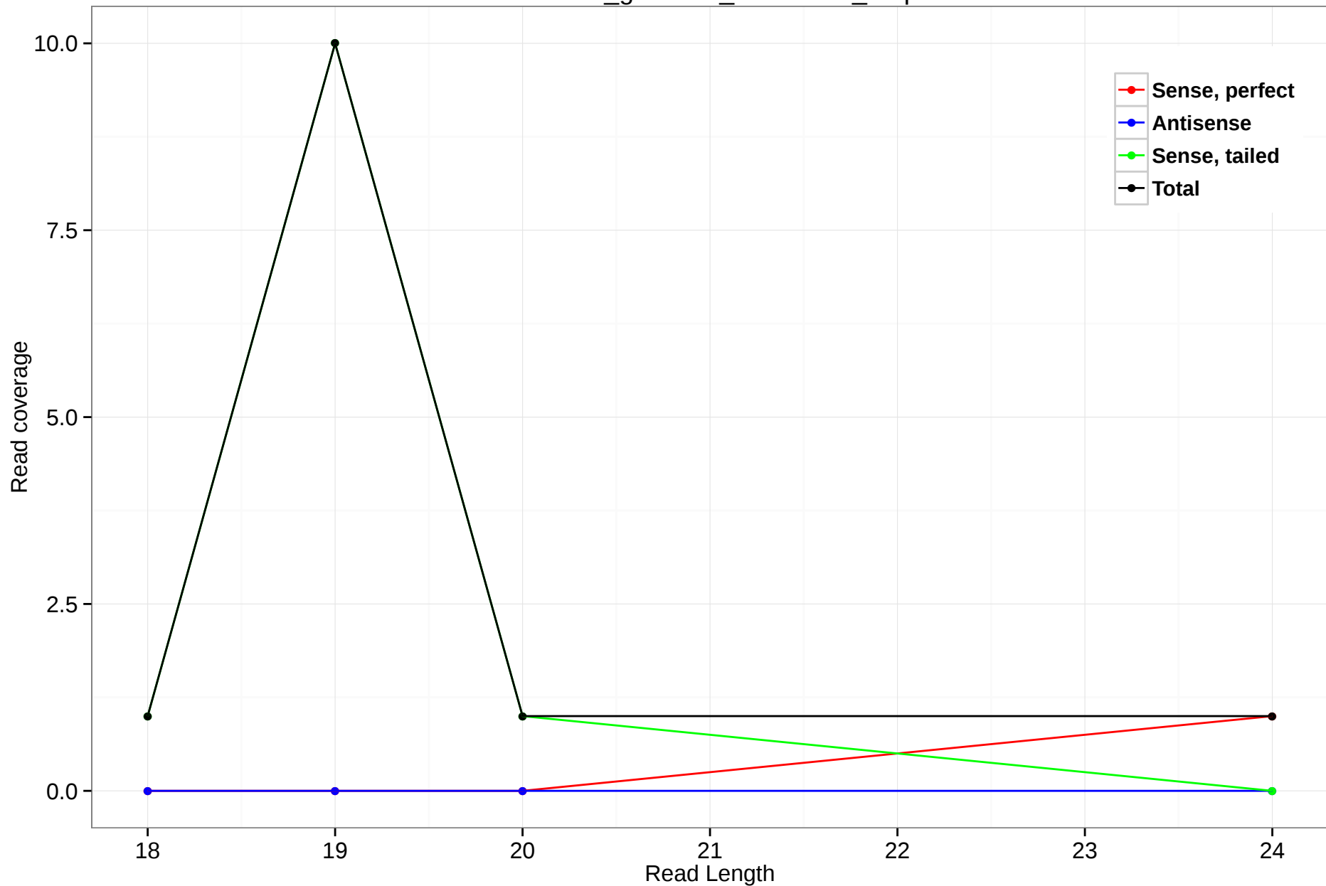
rheMac3_genscan_chr7.2567_1.3p
