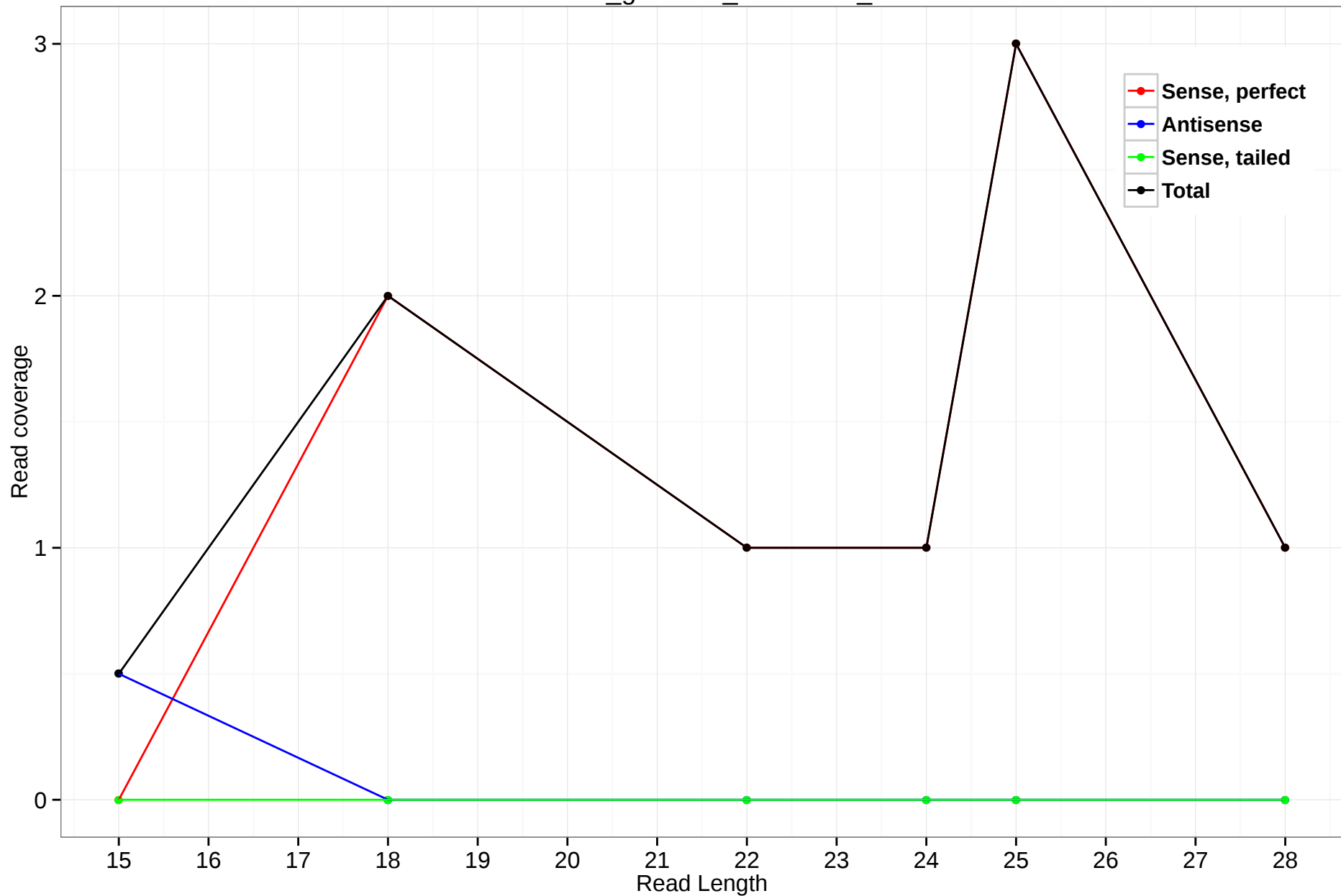
rheMac3_genscan_chr7.2533_27
