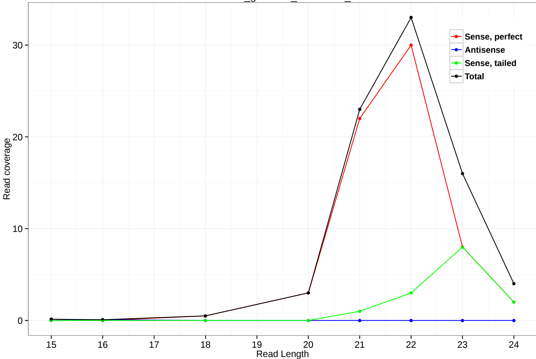
rheMac3_genscan_chr7.2533_18
