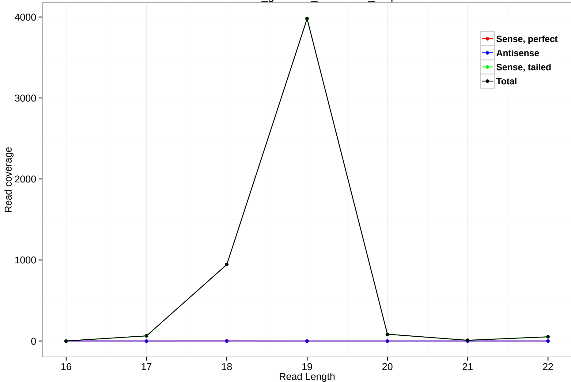
rheMac3_genscan_chr7.2516_6.5p
