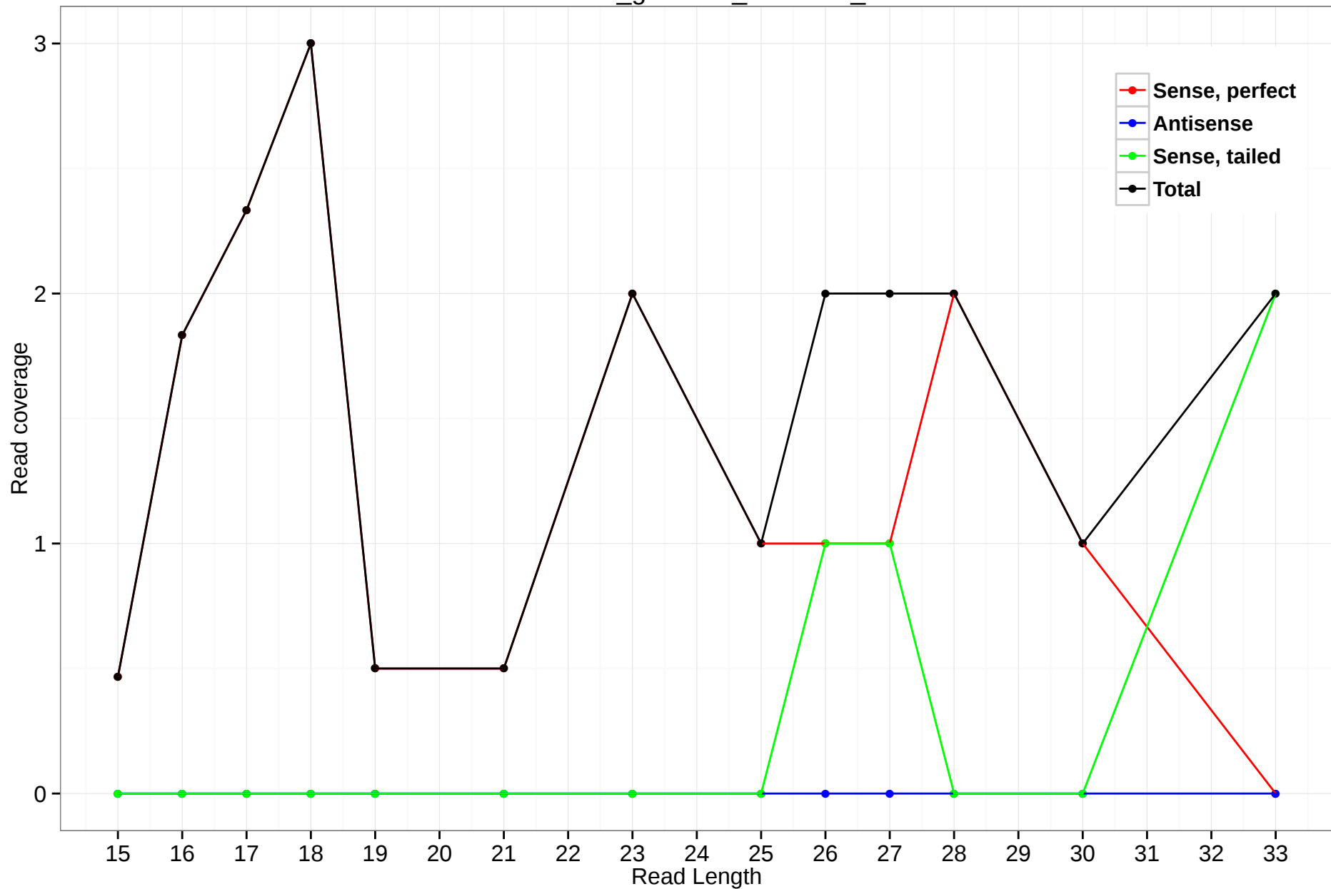
rheMac3_genscan_chr7.250_2
