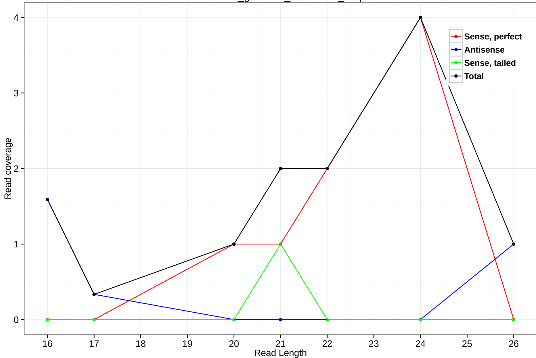
rheMac3_genscan_chr7.2475_4.3p
