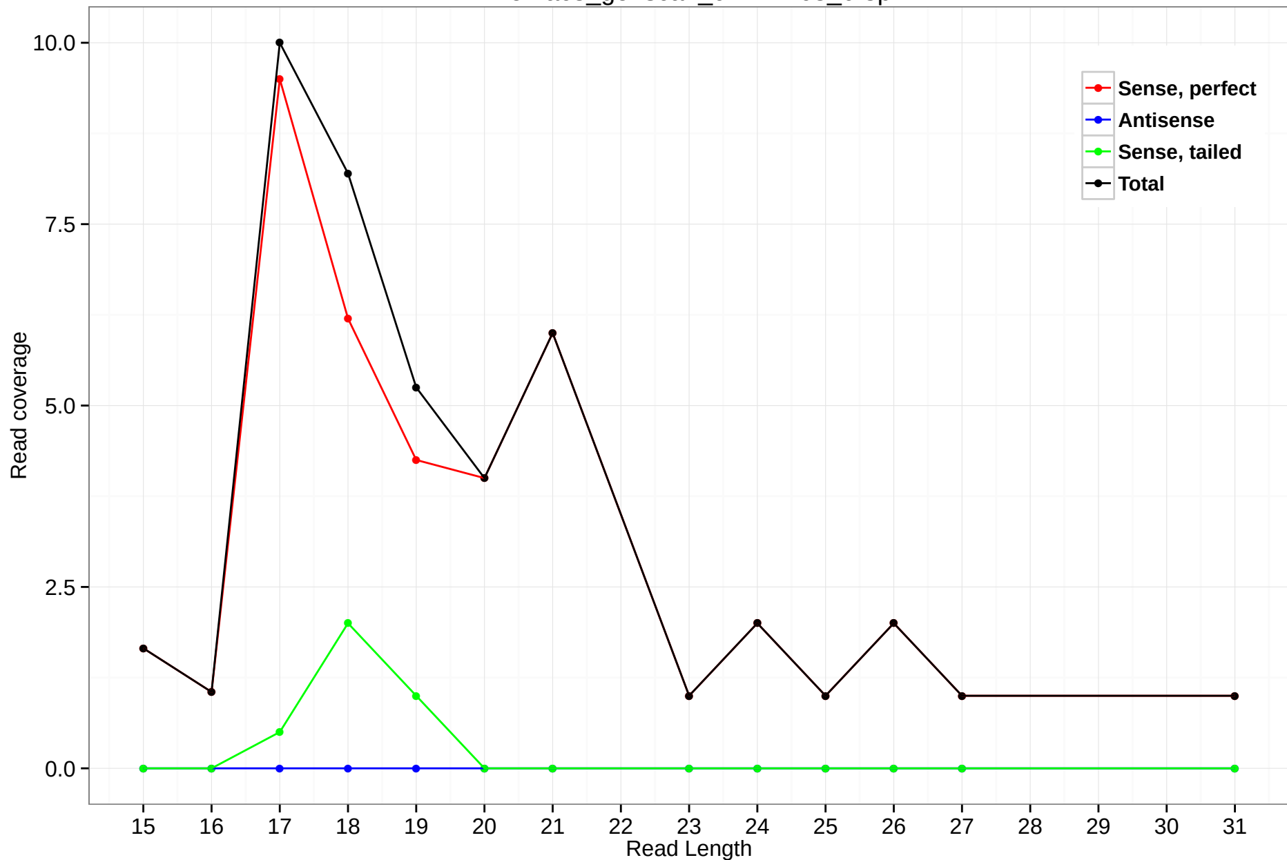
rheMac3_genscan_chr7.2463_0.3p
