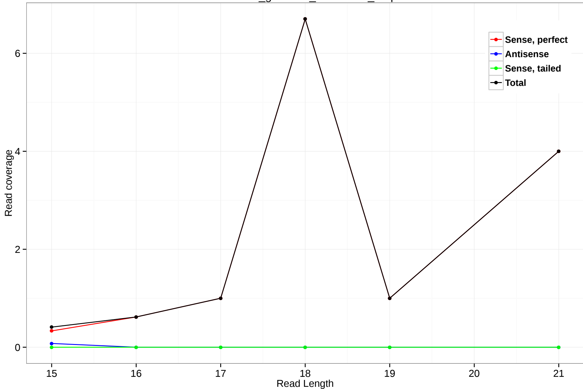
rheMac3_genscan_chr7.2406_0.3p
