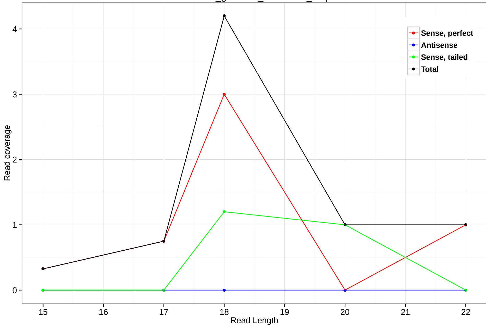
rheMac3_genscan_chr7.2354_2.5p
