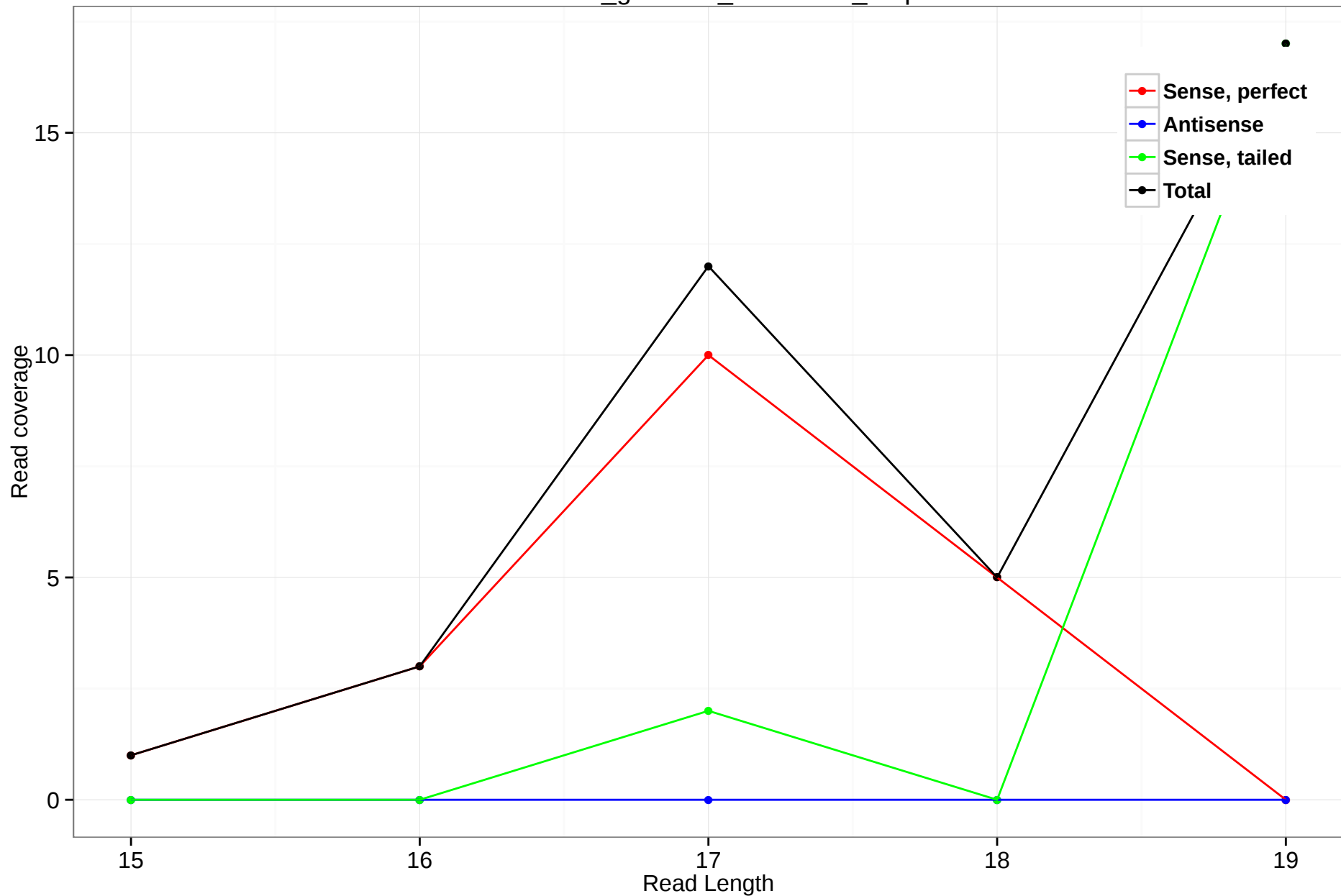
rheMac3_genscan_chr7.2290_5.5p
