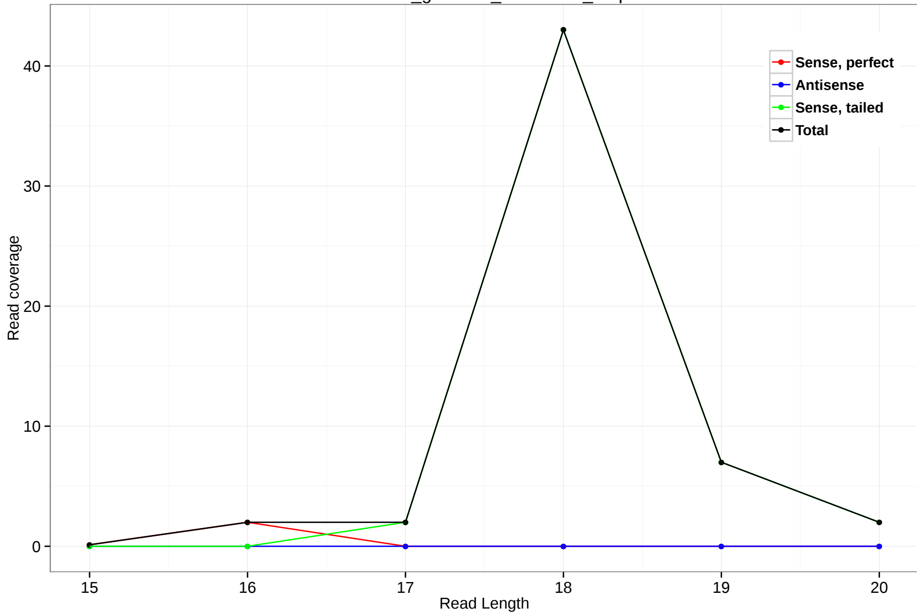
rheMac3_genscan_chr7.1996_4.5p
