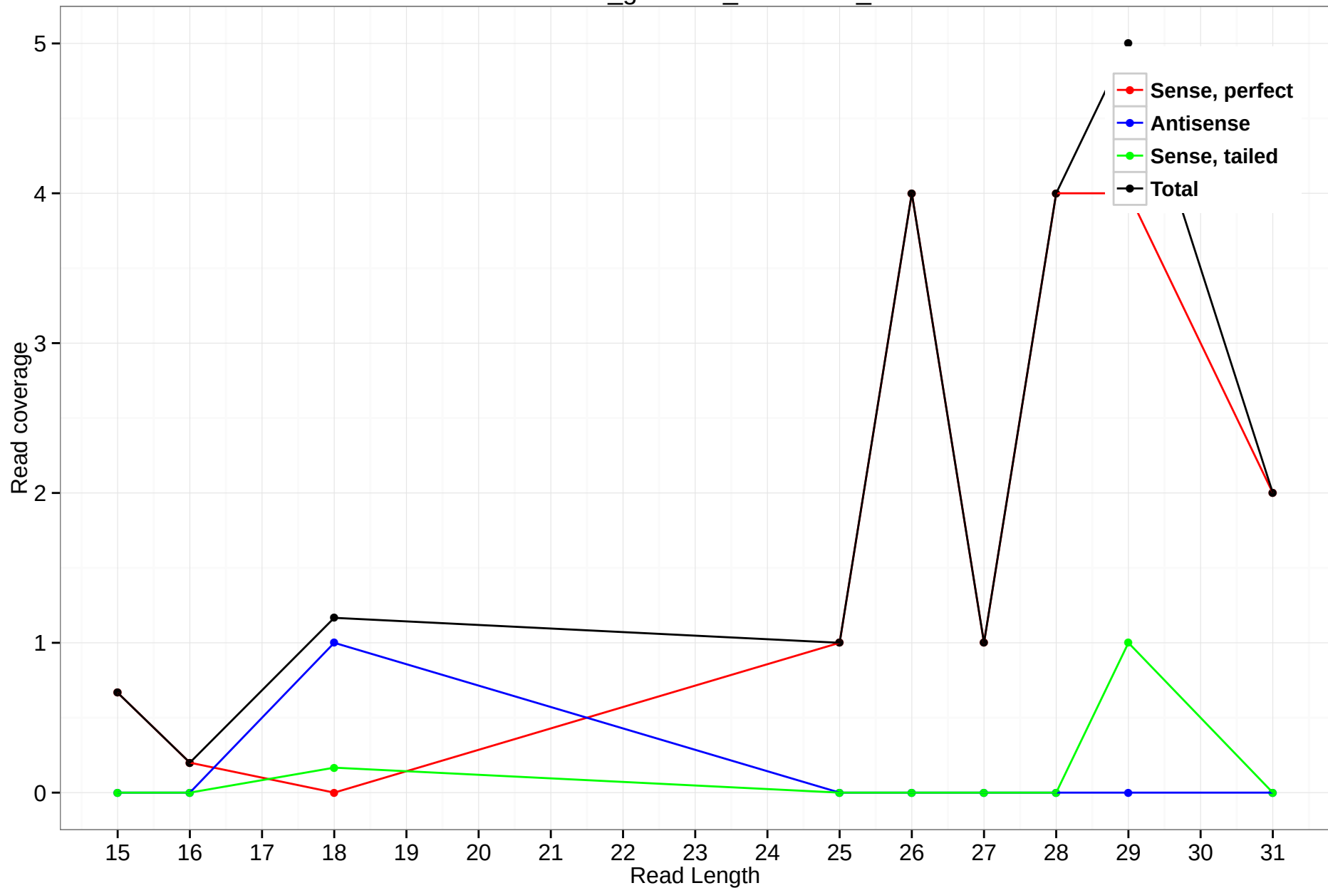
rheMac3_genscan_chr7.1806_2
