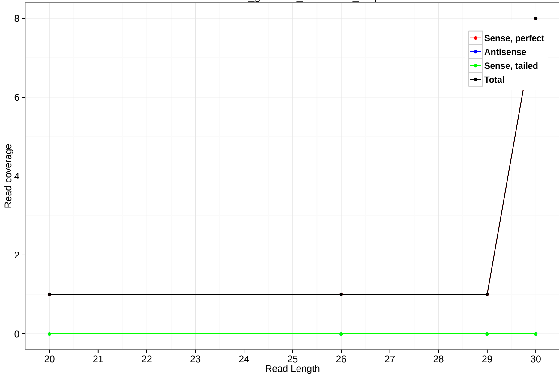
rheMac3_genscan_chr7.1757_2.5p
