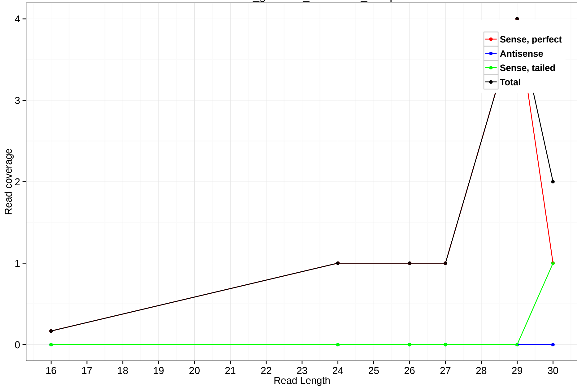
rheMac3_genscan_chr7.1755_27.3p
