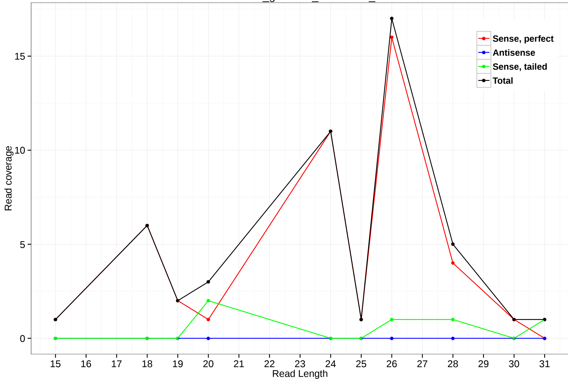
rheMac3_genscan_chr7.1753_0
