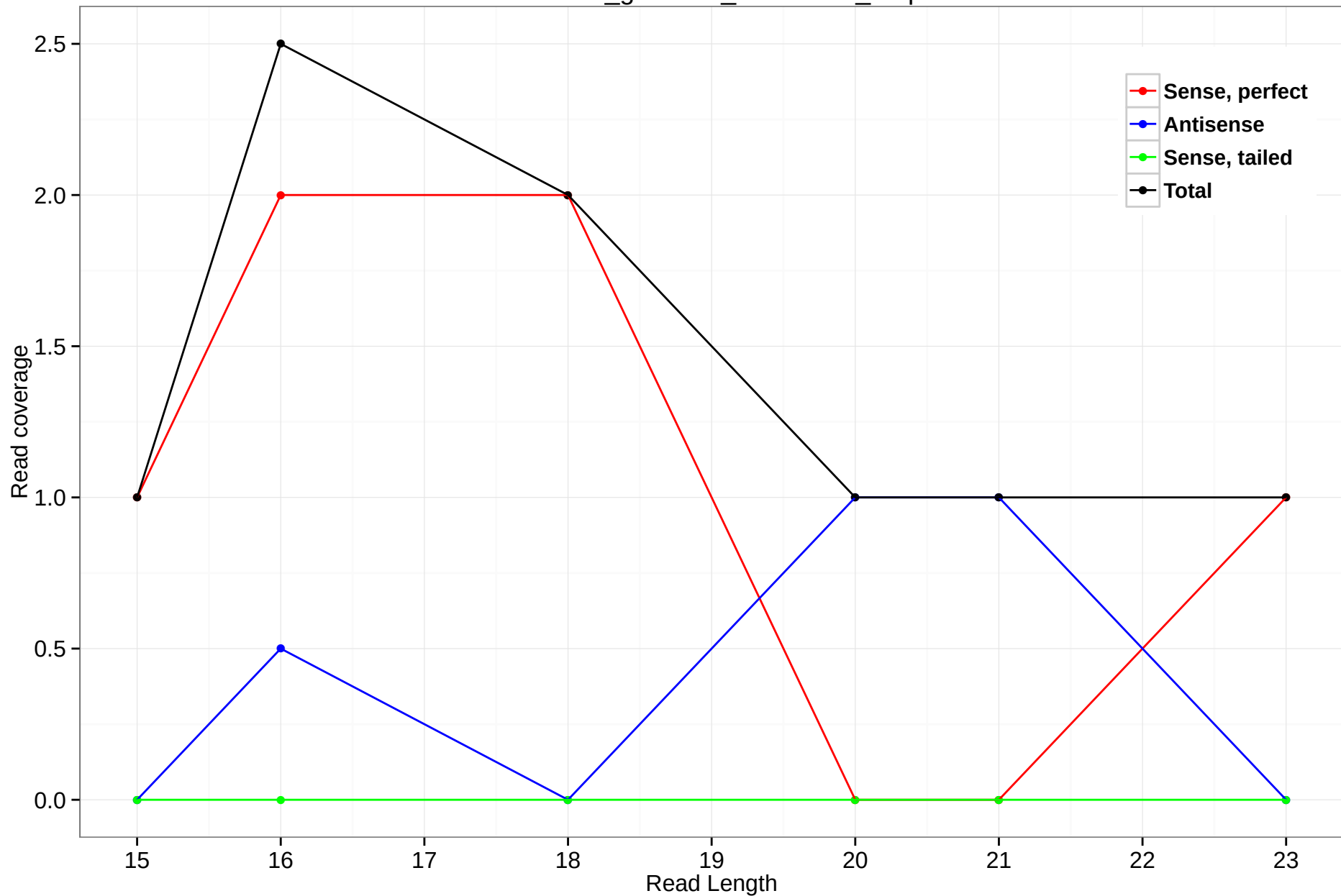
rheMac3_genscan_chr7.1749_4.5p
