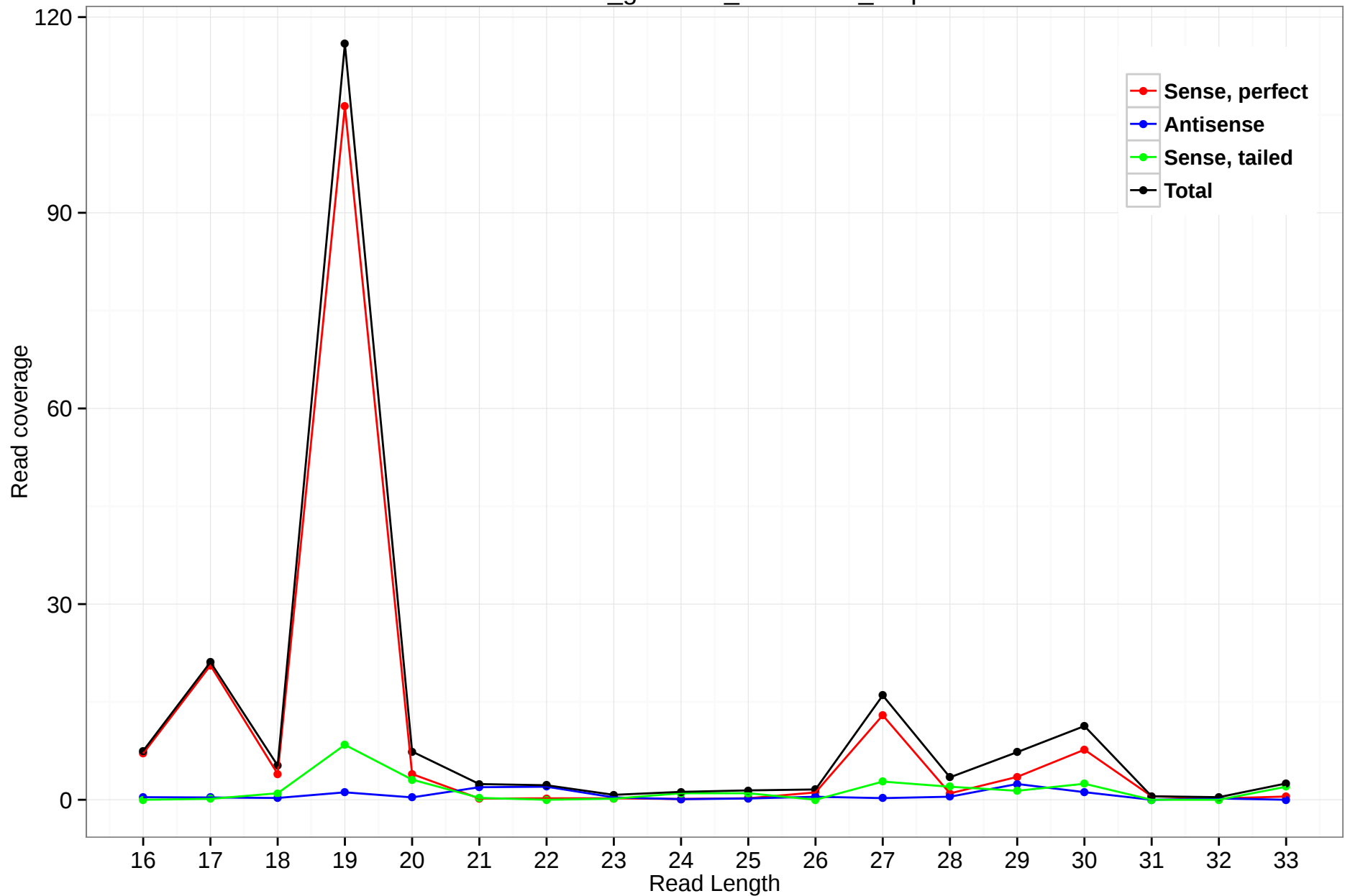
rheMac3_genscan_chr7.1623_5.3p
