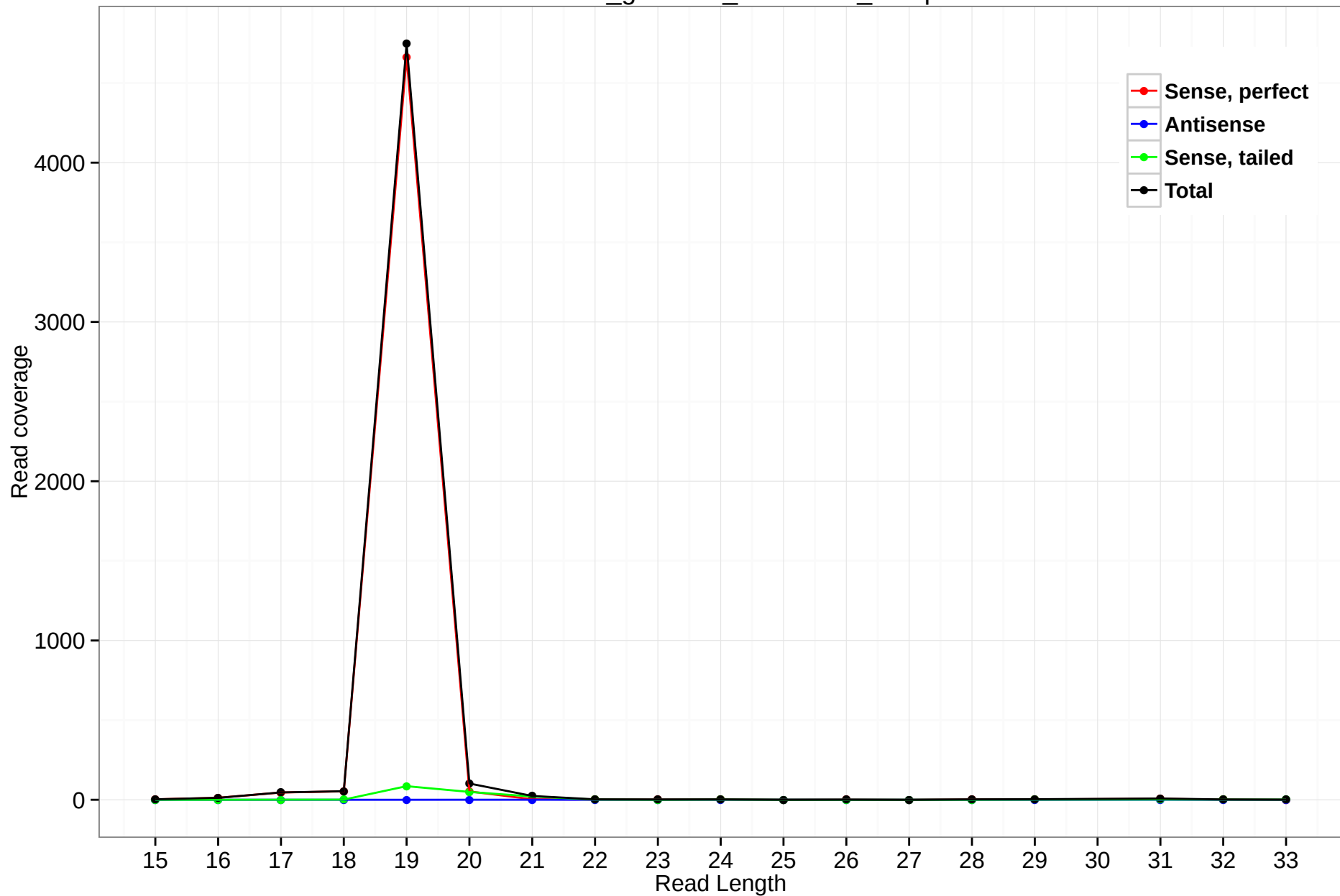
rheMac3_genscan_chr7.1623_12.5p
