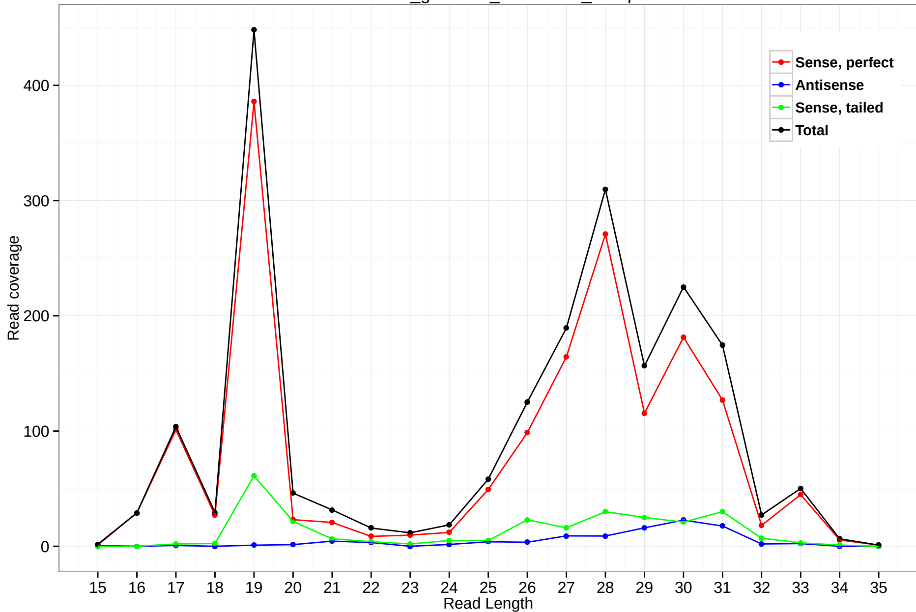
rheMac3_genscan_chr7.1623_11.5p
