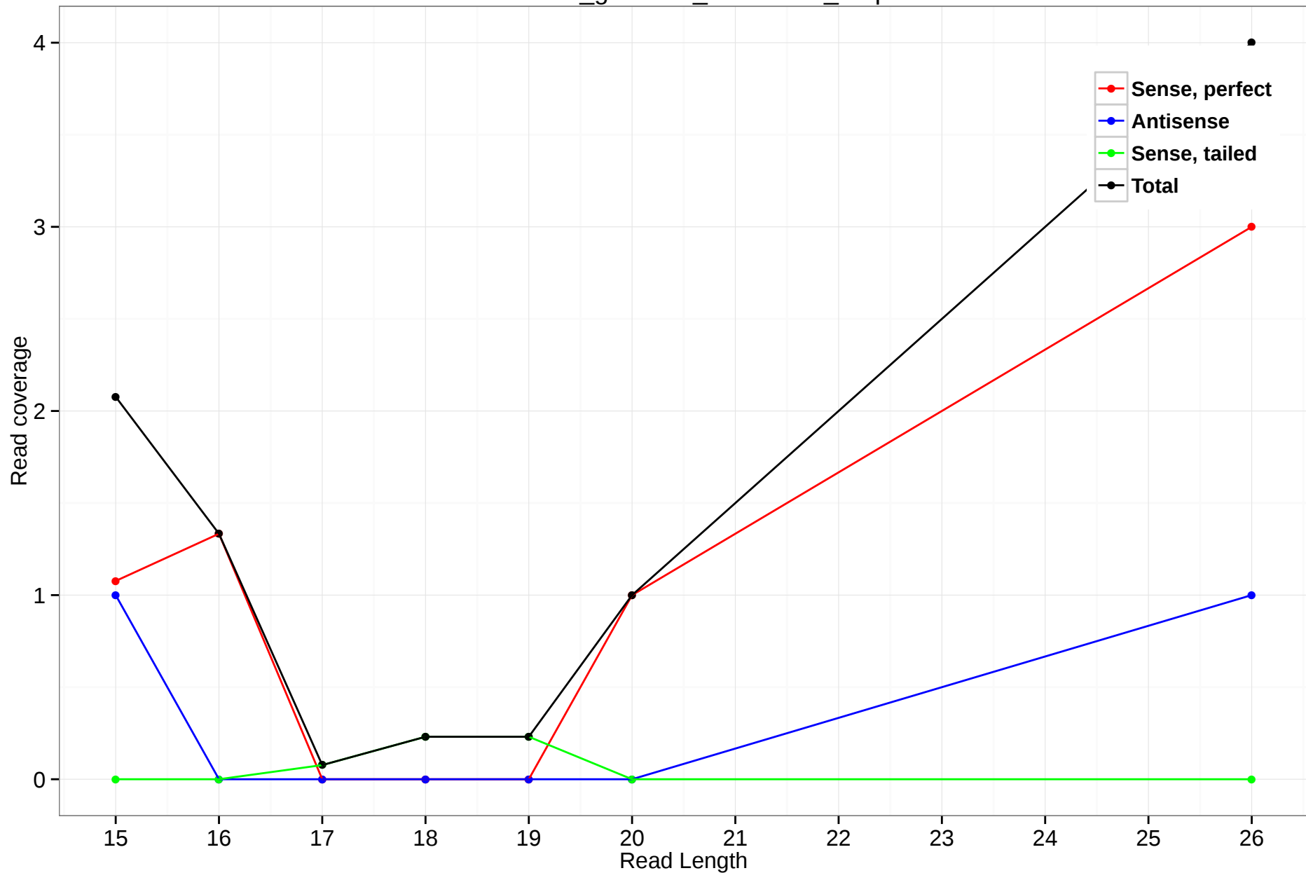
rheMac3_genscan_chr7.1620_0.5p
