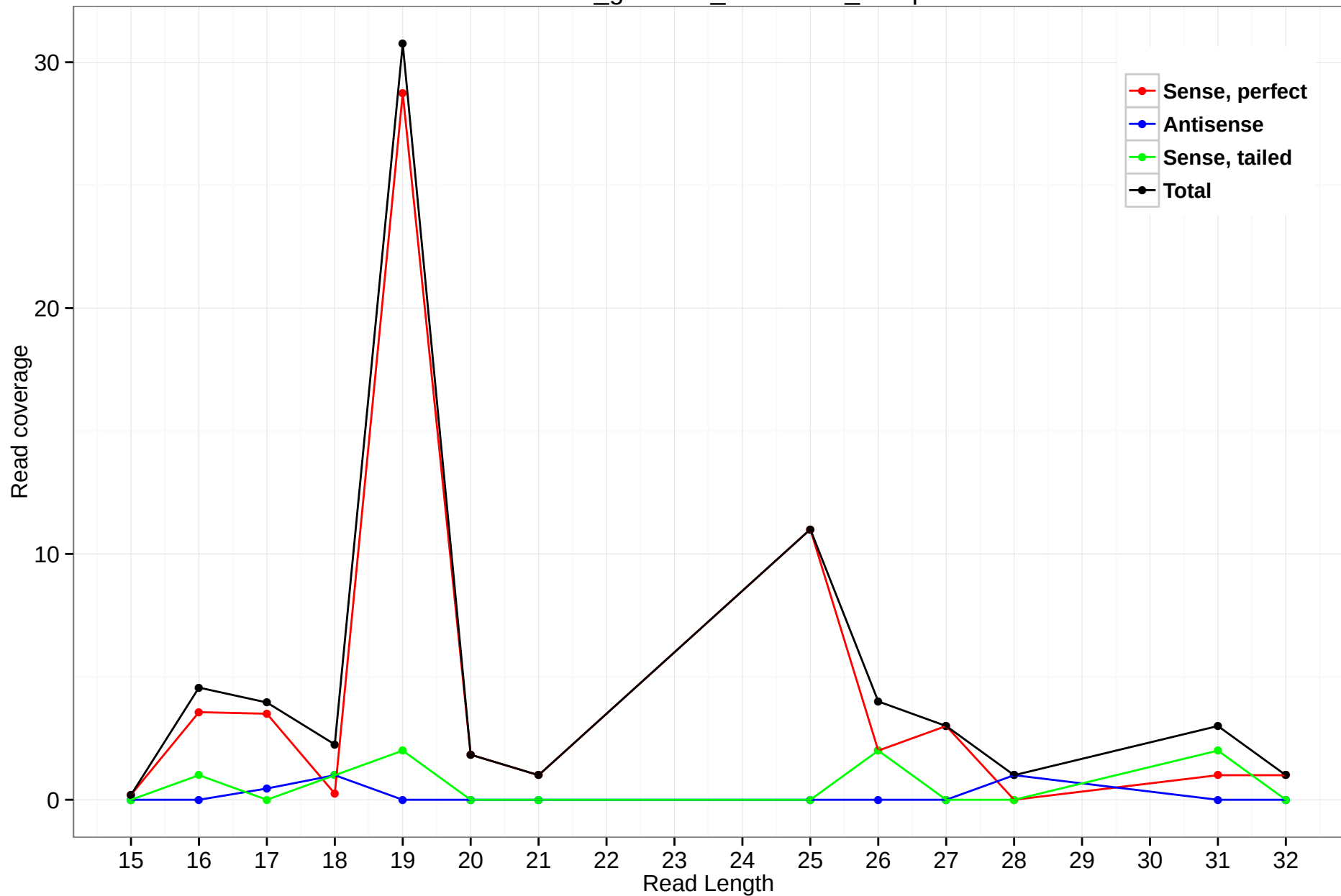
rheMac3_genscan_chr7.1580_11.5p
