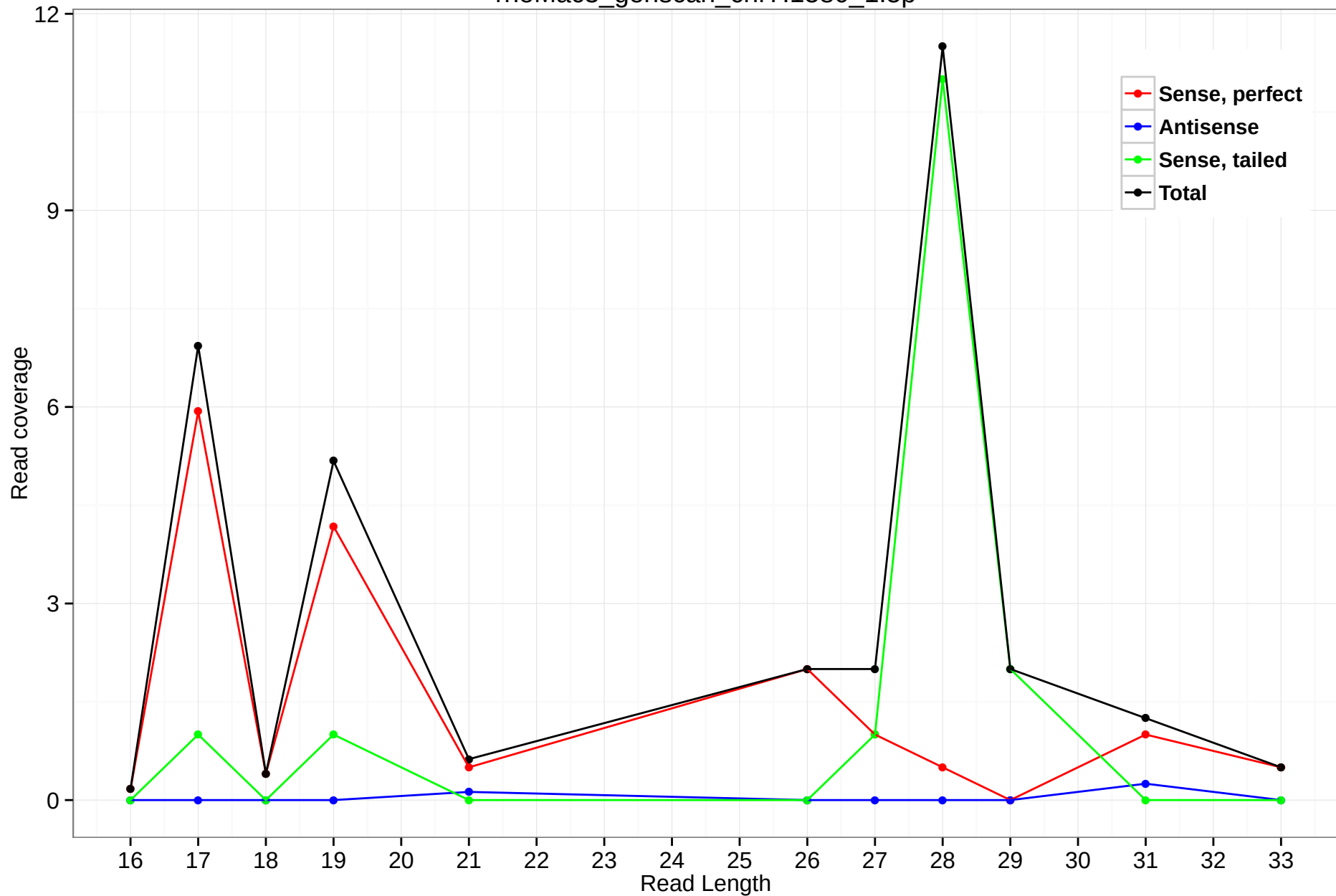
rheMac3_genscan_chr7.1580_1.5p
