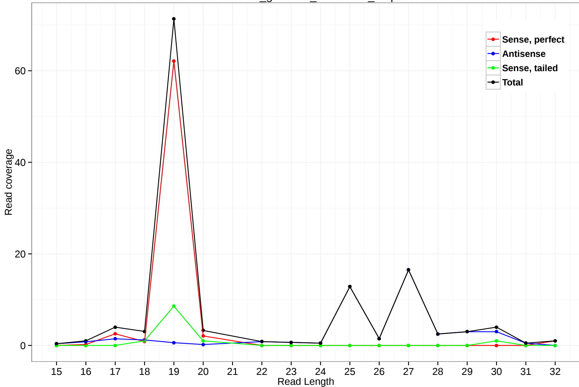
rheMac3_genscan_chr7.1580_1.3p
