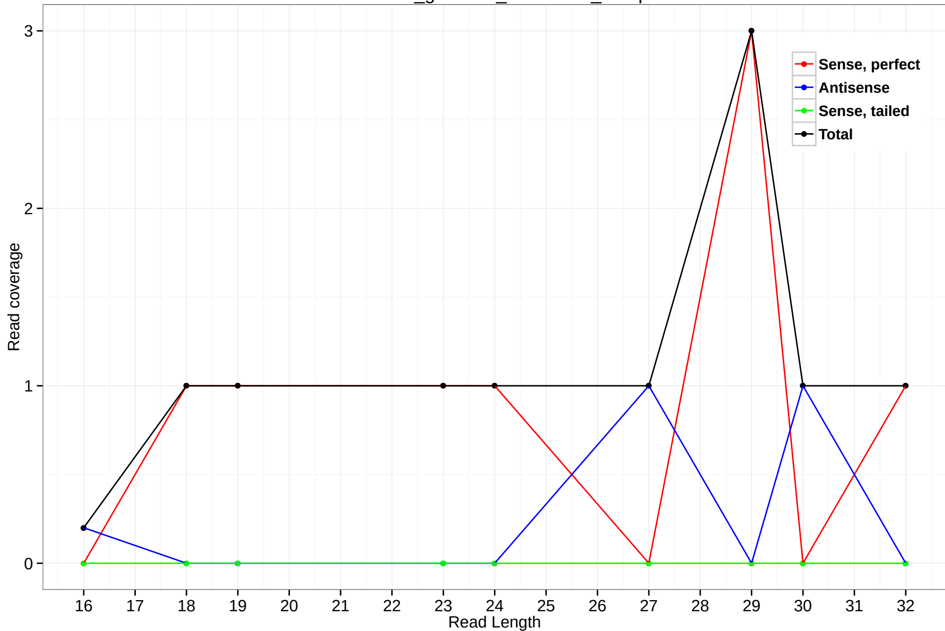
rheMac3_genscan_chr7.1563_12.5p
