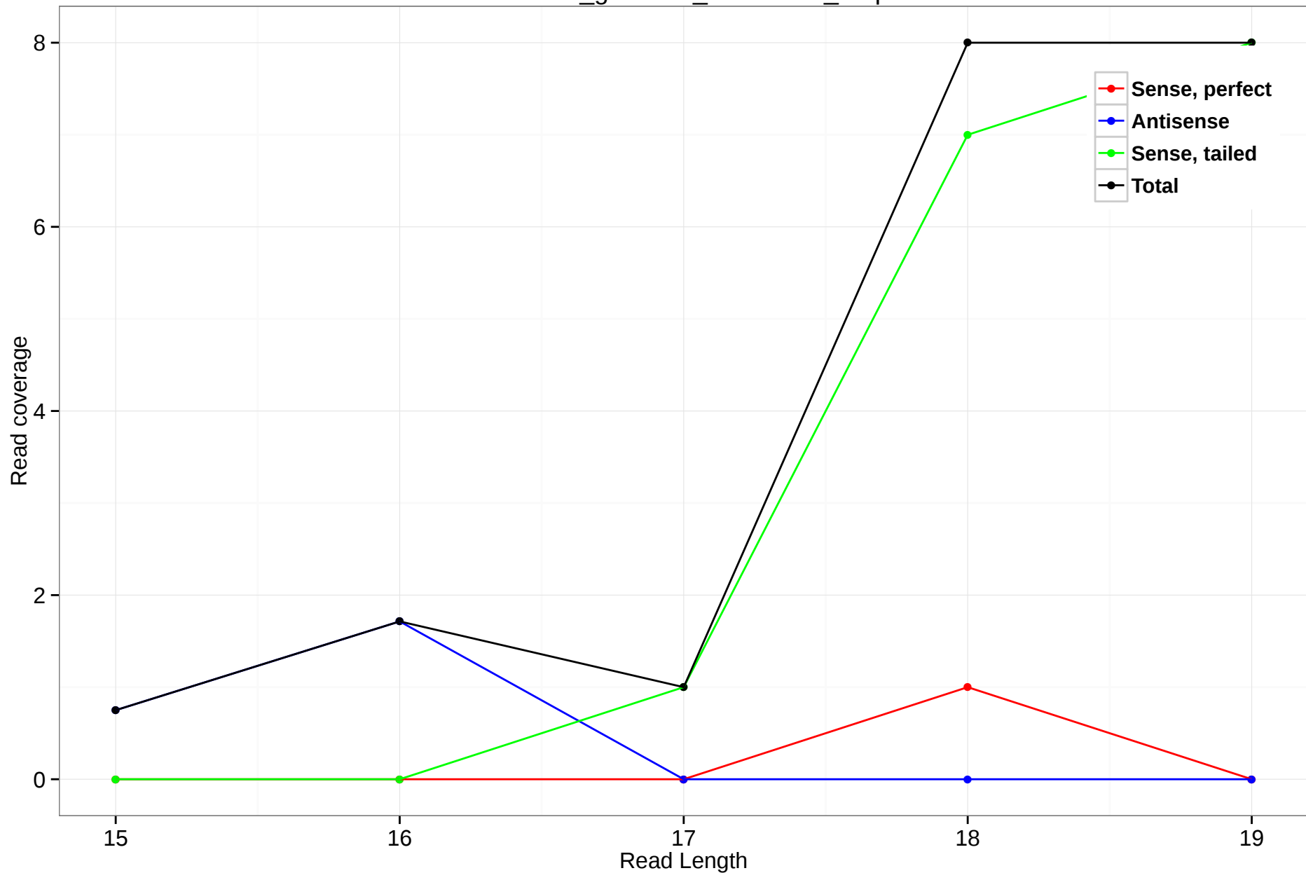
rheMac3_genscan_chr7.1557_5.3p
