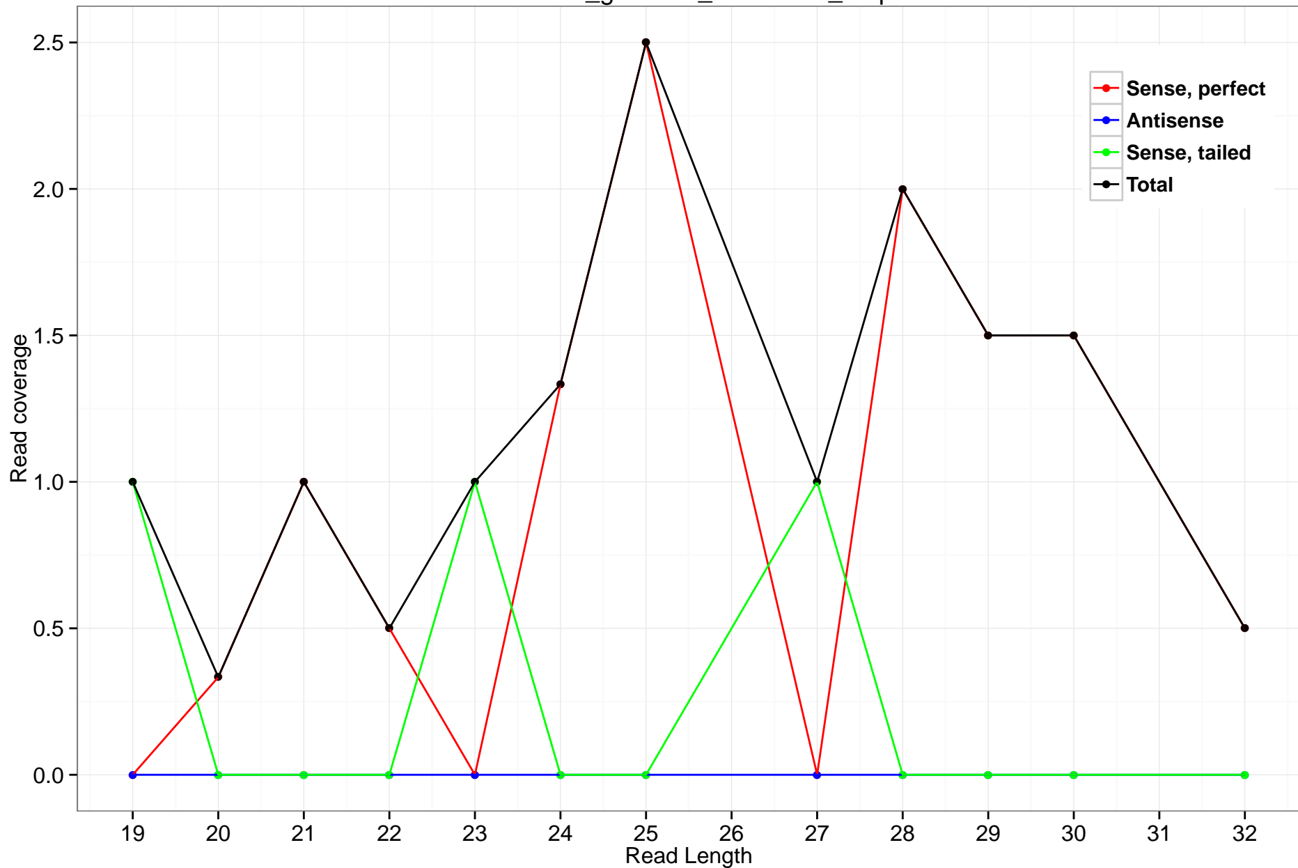
rheMac3_genscan_chr7.1546_0.5p
