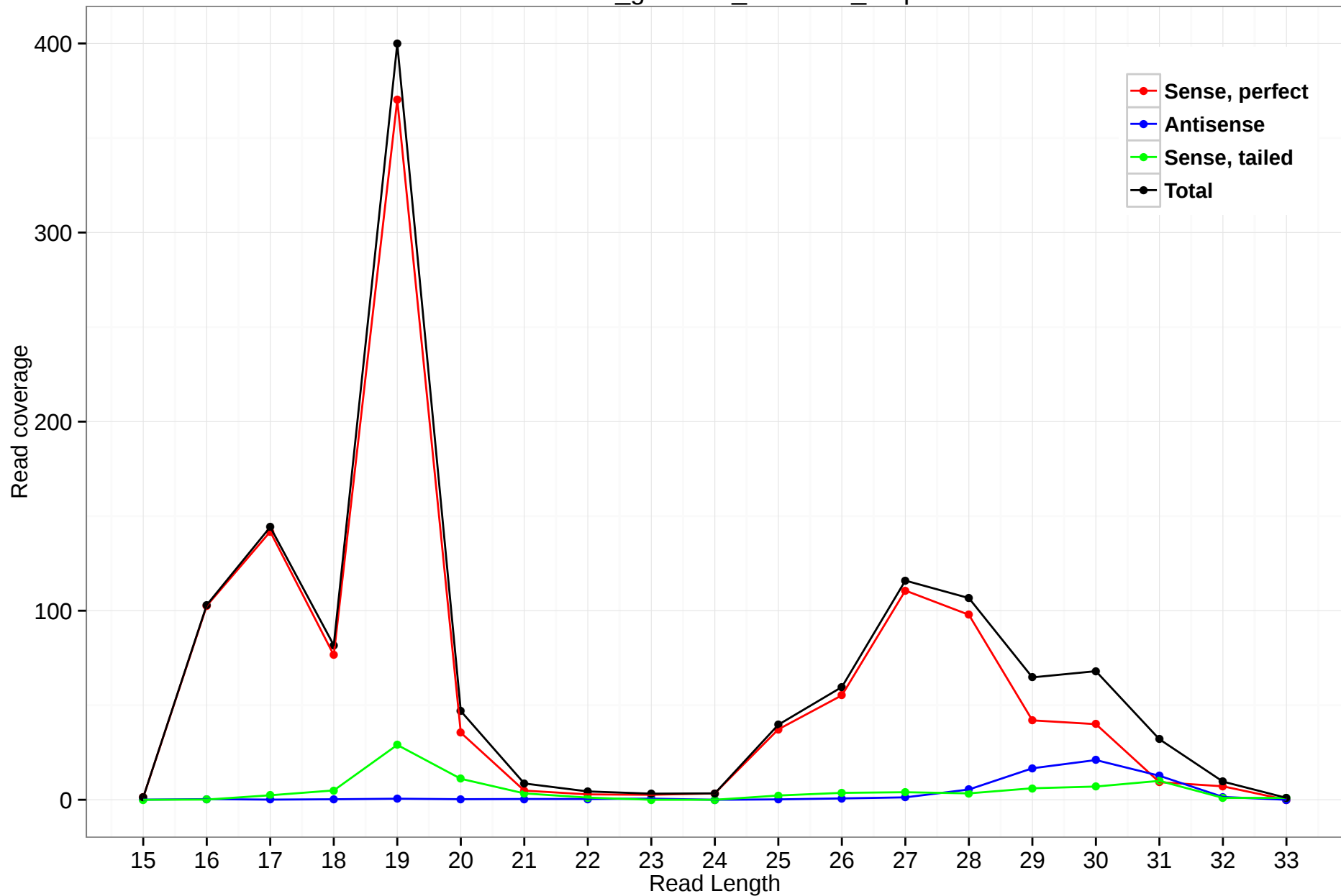
rheMac3_genscan_chr7.151_5.3p
