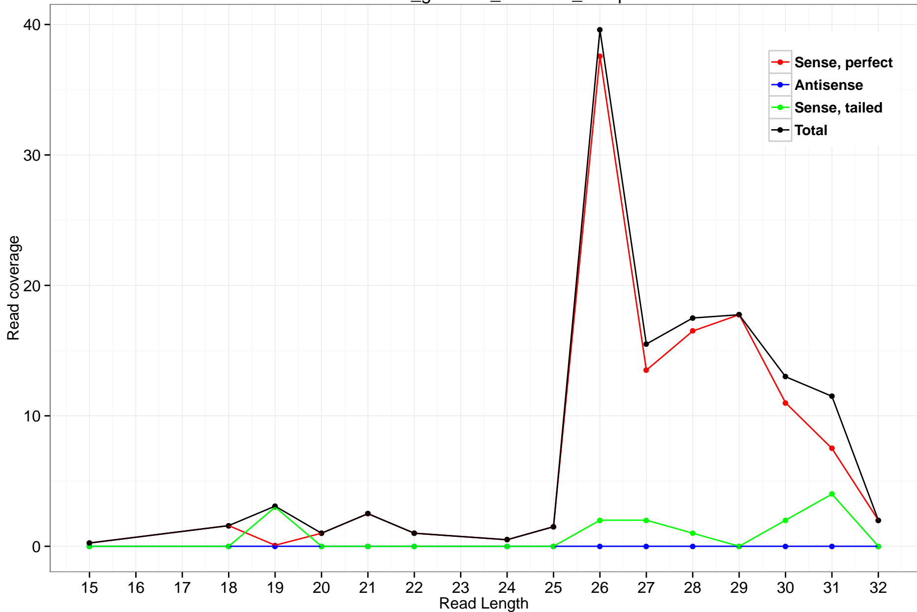
rheMac3_genscan_chr7.151_15.5p
